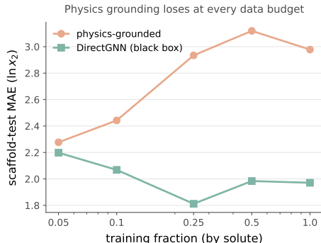
Figure 8: Data-efficiency curve. The physics-grounded arm (salmon) trails the DirectGNN black box (teal) at every training-data fraction; the gap is smallest at the least data and large thereafter—the opposite of the low-data advantage a physics prior is supposed to provide.
