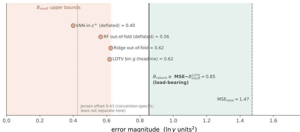
Closure-insufficiency bounds, deployed residual-only COSMO-SAC ( n = 60 ): B_{\text{closure}} dominates (leakage-immune bound)
