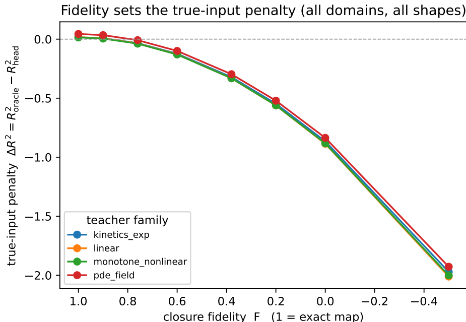
Figure 5: Reproducible closure-fidelity dial ( run_fidelity_dial.py ). As the closure is made more misspecified (fidelity F decreasing from 1), the true-input penalty \Delta R^2 = R^2_{\text{oracle}} - R^2_{\text{head}} grows monotonically, and the same ordering holds across four non-chemistry teacher families (linear, monotone, kinetics-exponential, PDE-field) and six misspecification functional forms. The effect is a property of the fidelity magnitude, not of any one domain or deformation. The real COSMO-SAC closure sits well inside the misspecified regime ( F \lesssim 0.4 )—the sign and rough magnitude of the empirical paradox, not a precise fidelity value.
