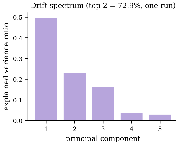
Figure 7: Explained-variance spectrum of the fine-tuning drift on the 44 matched molecules (companion run). Caveat: this share carries no matched null (text).
