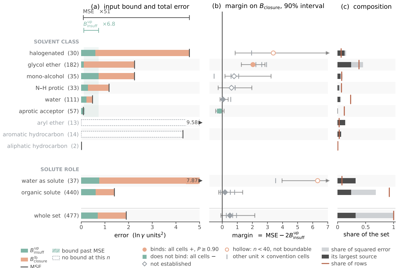
Figure 5: Where the closure binds , by solvent class and by solute role, on the broad IDAC set (477 rows, 185 pairs, 78 solutes, 36 solvents). Bars, points and shares are at the row unit under the deployed residual-only convention, at one estimator cell for every stratum—eight equal-count bins of g(z^*) with the Bessel within-bin variance. (a) each stratum’s input-insufficiency bound and its total error; (b) the margin between them with its 90% two-way cluster-bootstrap interval, the other three unit \times convention cells as grey ticks; (c) each stratum’s share of the set’s squared error, the part carried by its largest source publication drawn dark. Grade: likely for the glycol ethers, positive in all four cells at P > 0.95 ; open for every other row, the aggregate included. Caveat: a hollow marker is a stratum below n=40 , three classes carry no bound at any n , and the two hollow positive cells rest on two publications and on one, which panel (c) shows.
