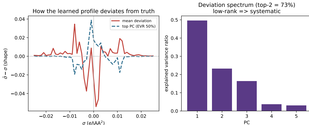
Figure 10: The learned \sigma -profile is a systematic closure-compensating surrogate, not the physical profile. Left : the mean deviation \hat{\sigma} - \sigma (and its dominant PCA mode) transfers area out of the nonpolar bins ( \sigma \approx 0 ) into the polar wings—the network makes molecules look more polar than they are, inflating the segment interactions the misspecified closure under-weights. Right : the deviation spectrum is low-rank (top-two modes 73%; noise would be flat at \approx 4\% ), i.e. the distortion is systematic. A single affine distortion transfers 3.3\times better than identity out-of-sample, so \hat{\sigma} is a transferable closure-compensating surrogate of \sigma , not \sigma with noise (confound-free one-model control, n=44 matched VT-2005 molecules).
