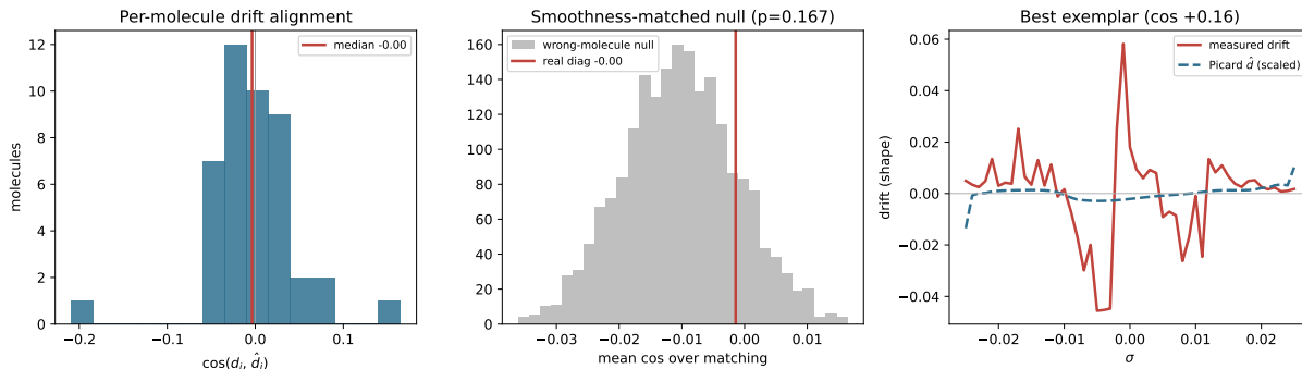
Figure 9: The compensating drift is not the closure’s linear-response inverse. Left : per-molecule cosine between the measured drift \hat{\sigma} - \sigma and the first-order closure compensation J^+(m - g) is centred on zero (median -0.00 ). Middle : the smoothness-matched wrong-molecule control—each molecule’s drift aligned against every other molecule’s predicted drift, all equally smooth—places the true diagonal squarely inside the null ( p=0.17 ), so any weak alignment is generic smoothness, not molecule-specific closure geometry. Right : the best-aligned exemplar, showing that even the strongest case is not tracked by the Picard prediction. The surrogate is structured but not readable from the closure.
