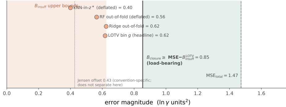
Figure 8: One-sided bounds on the closure-insufficiency split under the deployed residual-only COSMO-SAC convention—the configuration the model actually runs. The load-bearing, convention-independent bound B_{\text{closure}} \geq \text{MSE} - B_{\text{insuff}}^{\text{LOTV}} \approx 0.85 exceeds every valid B_{\text{insuff}} upper bound (salmon region); the white gap is a separation that needs no smoothness assumption, and the teal region is the certified closure share of the total error ( \text{MSE} = 1.47 ). We headline the law-of-total-variance (LOTV) binning bound because it conditions on the scalar g(z^*) and is immune to the near-duplicate leakage that deflates the z^* -neighbour estimators ( k -NN, RF; §6.2). The assumption-free Jensen constant-offset bound is convention-specific and inverts here ( 0.43 < 0.62 , dotted), which is why we do not lean on it.
