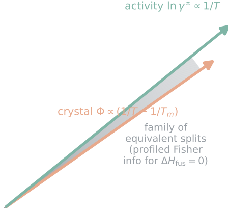
Figure 4: Why the crystal/activity split is non-identifiable from solubility. (a) As functions of 1/T the crystal direction \Phi and the activity direction \ln \gamma^\infty are nearly collinear, so a whole band of crystal/activity splits fits the data equally well (the profiled Fisher information for \Delta H_{\text{fus}} is zero, Lemma 1). (b) An external single-component label points off that axis and collapses the band to a point, pinning the split—the mechanism behind the aux-stream grounding, with the measured Cramér–Rao drop on \Delta H_{\text{fus}} .
