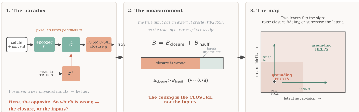
Figure 1: The paper in one view. A learned encoder h predicts a physical latent—a molecular \sigma -profile—that a fixed COSMO-SAC closure g (no fitted parameters) turns into a solubility. (1) The paradox : replacing the learned \hat{\sigma} with the external quantum-chemical reference \sigma^* (VT-2005) makes the prediction worse than a free learned head—so which is wrong, the closure or the inputs? (2) The measurement : because the latent has an external oracle, the true-input excess risk splits exactly into a closure-misspecification part B_{\text{closure}} and an input-insufficiency part B_{\text{insuff}} ; on the matched low- \gamma set the closure binds ( B_{\text{closure}} > B_{\text{insuff}} , P \approx 0.78 ). (3) The map : two levers move the ceiling—raising closure fidelity (COSMO-SAC-2010/dsp) or supervising the latent toward truth (TeNNet-SAC)—so whether grounding helps is governed by two axes, closure fidelity and latent supervision.
