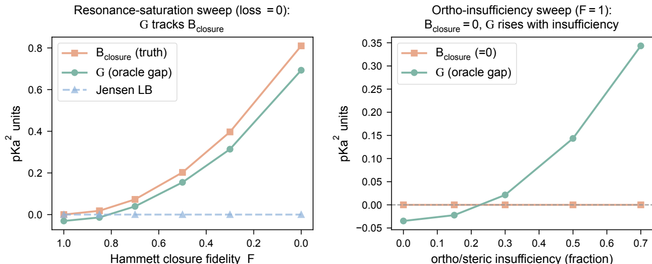
Figure S11: \text{pKa} through a Hammett LFER on a construction with known ground-truth channels. Left : closure fidelity varied with a sufficient intermediate; grounding gap \mathcal{G} , closure bias B_{\text{closure}} , and the assumption-light Jensen bound. Right : an ortho/steric insufficiency channel varied with a well-specified closure; B_{\text{closure}} = 0 at each knob while \mathcal{G} rises with the insufficiency fraction, crossing zero near 0.25.
