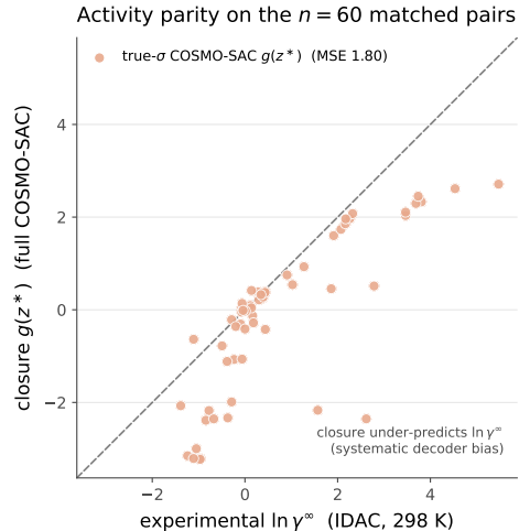
Figure 7: Activity-coefficient parity on the n=60 matched pairs. The reference- \sigma COSMO-SAC closure g(z^*) (salmon) falls systematically below the diagonal at larger \ln \gamma_2^\infty , under-predicting the activity coefficient (MSE 1.80, full convention). This systematic downward bias is the visible form of the decoder misspecification B_{\text{closure}} ; for reference a flexible regressor of \ln \gamma_2^\infty on the same reference profiles reaches the irreducible-variance floor (MSE \approx 0.40 , our B_{\text{insuff}} estimator; §6.2), so the closure’s excess over that floor is B_{\text{closure}} .
