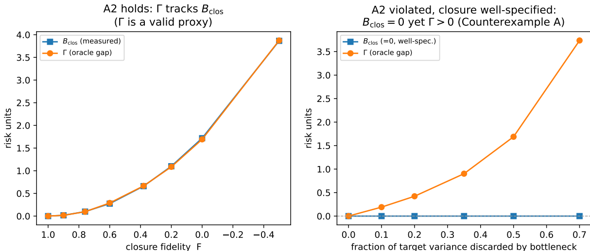
Figure 12: The grounding gap \Gamma is a symptom, not a certificate (§4.3; run_fidelity_dial.py ). Left: when the intermediate is sufficient (A2 holds), \Gamma tracks the closure bias B_{\text{closure}} as fidelity varies, so Theorem 1’s proxy is valid. Right: with a well-specified closure ( B_{\text{closure}} = 0 ) but a lossy intermediate (A2 fails), \Gamma > 0 and grows with the discarded variance—a positive grounding gap from pure input insufficiency (the worked counterexample in the proof of Theorem 1, App. B). Hence certification of closure-dominance rests on the decomposition, which needs neither assumption.
