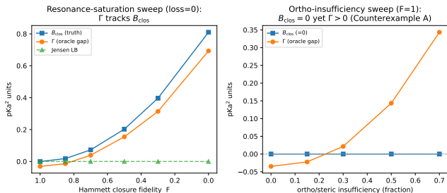
Figure 8: The diagnostic transfers to a second real closure ( \text{p}K_a through a Hammett LFER), on a controlled construction with known ground-truth channels. Left: varying closure fidelity with a sufficient intermediate, the grounding gap \Gamma tracks the closure bias B_{\text{closure}} (the assumption-light Jensen bound is flat here because the misspecification carries no mean offset). Right: varying an ortho/steric insufficiency channel with a well-specified closure, B_{\text{closure}} = 0 throughout while \Gamma > 0 grows—the \text{p}K_a realization of the two-cause conflation of §4.3, and the reason certification rests on the decomposition, not on \Gamma .
