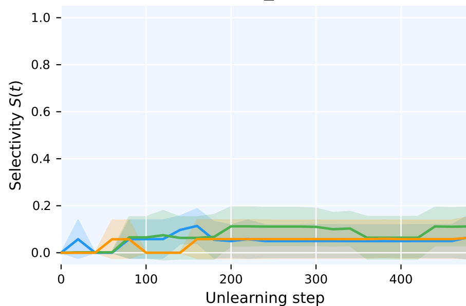
Acrobot no_clockwise
