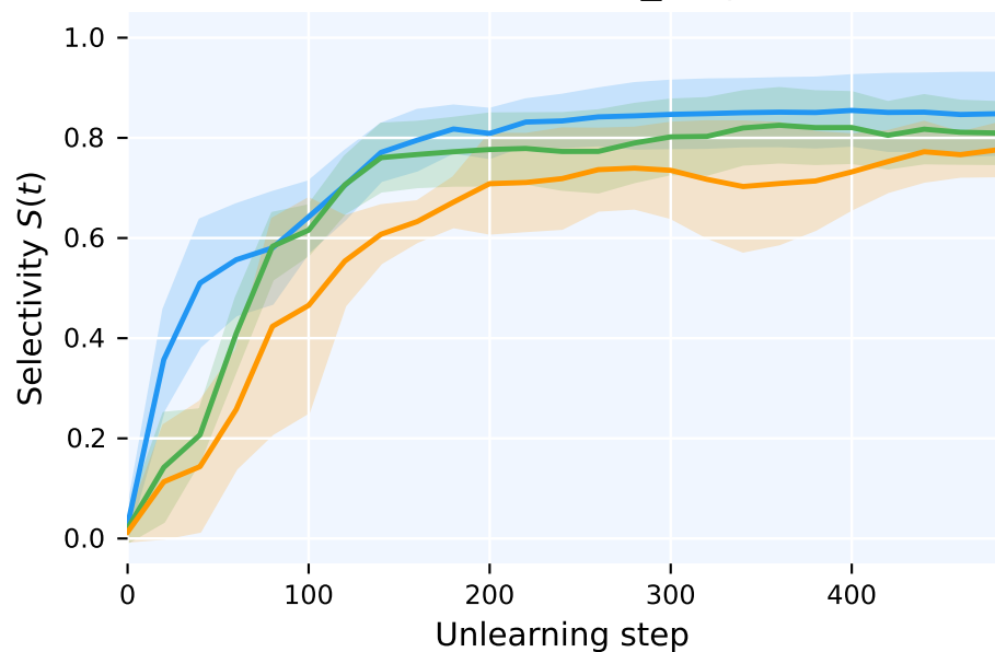
CartPole left_only
