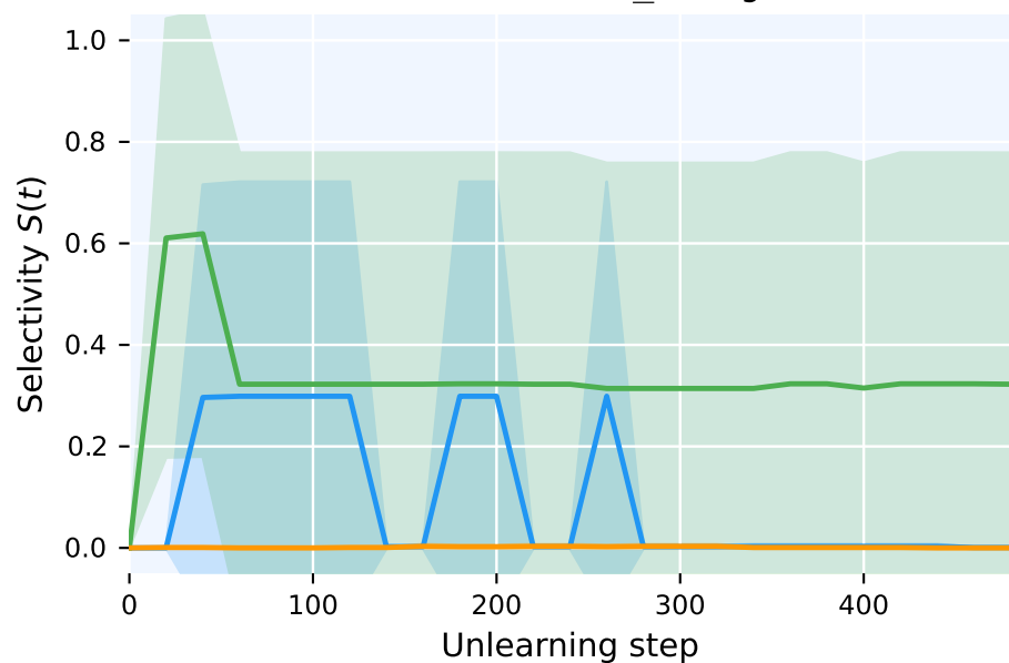
Acrobot slow_swing
