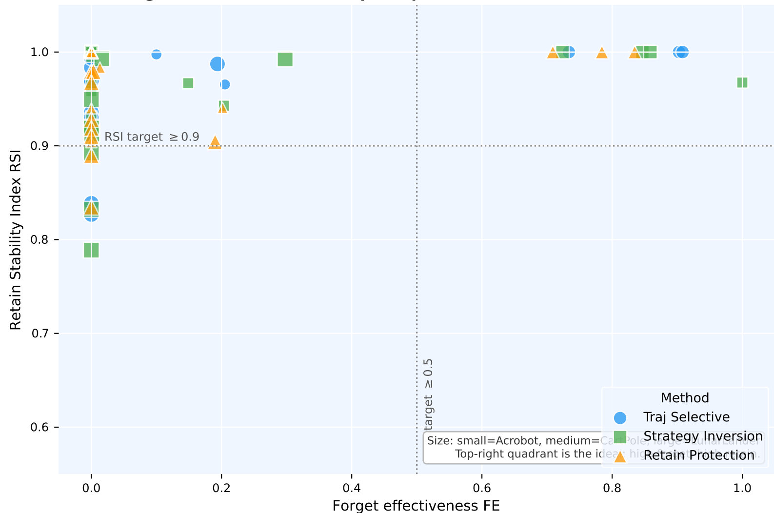
Forget-retain tradeoff: one point per seed; marker size encodes env
