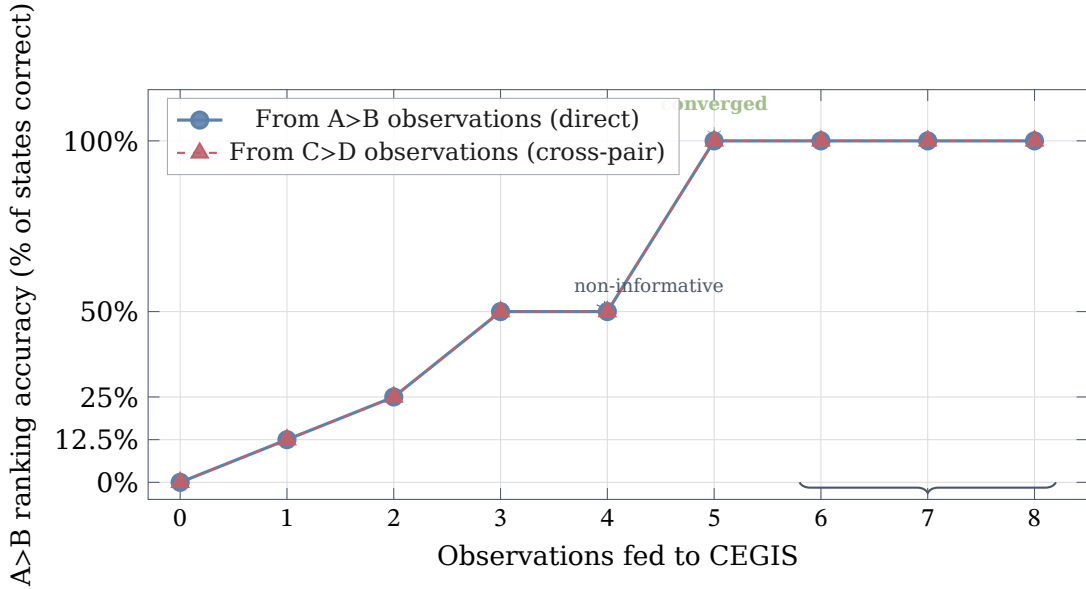
Figure 13: A>B ranking accuracy as C-vs-D (sub-optimal) observations accumulate. The blue circles (direct A>B observations) and red triangles (C>D cross-pair observations) produce identical curves —they overlap exactly. CEGIS receives the same PredObs values regardless of which pair was observed. Step 4 is non-informative (both surviving programs agree at that state). After step 5 the version space has converged; steps 6–8 are redundant. Every data point is verified by refl in Agda.
