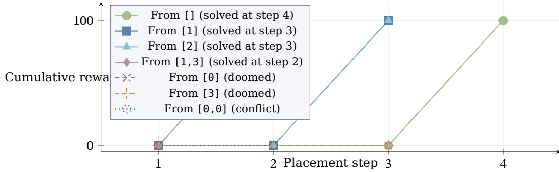
Figure 9: Cumulative reward along the synthesized policy’s trajectory for 4-Queens, starting from different partial placements. Valid starts ( [], [1], [2], [1,3] ) reach the solved state with reward 100; the closer the prefix to a solution, the sooner the reward appears. Doomed starts ( [0], [3] ) and conflicted starts ( [0,0] ) flatline at zero—no valid solution is reachable. Every data point is verified by refl .
