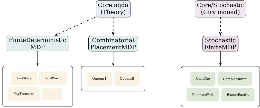
Fig. 3. Environment class hierarchy. Core provides theory; ECs provide reusable verification infrastructure; task groups contain domain-specific instantiations.
