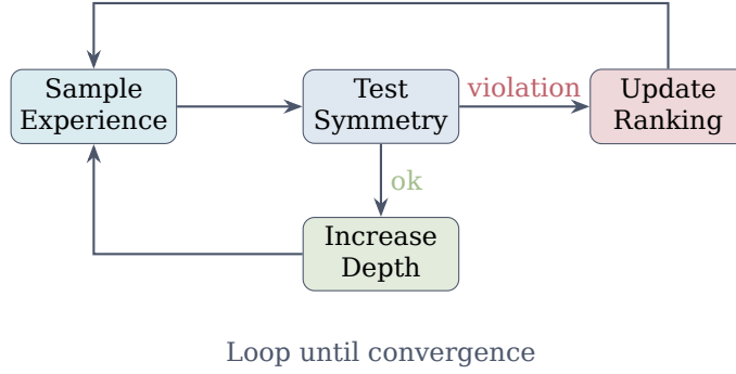
Fig. 4. The learning loop: sample, test for violations, update ranking, refine depth.
