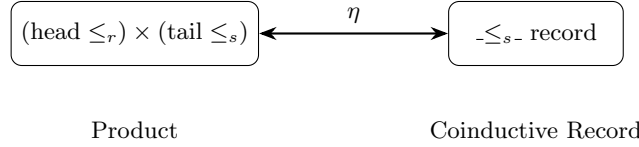
Figure 5: The product and record formulations are related by \eta -equivalence.
