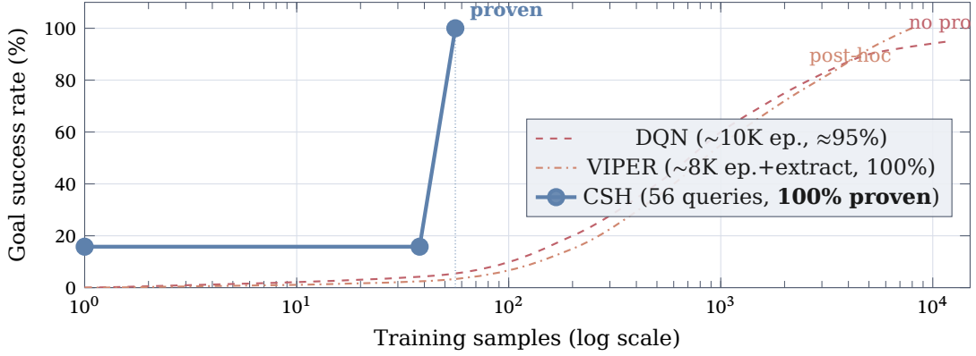
Figure 9: Goal success rate vs. training samples (log scale). CSH synthesis (solid blue) achieves provably 100% optimal performance in 56 oracle queries. VIPER [2] (dash-dotted orange) illustrates the distillation approach: a DNN is trained via standard RL, then compressed into a decision tree and verified post-hoc for specific properties—the total sample cost includes both training and extraction. A schematic DQN (dashed red) shows typical deep RL convergence. CSH’s step-like curve reflects the fundamental difference: synthesis produces a complete, proven policy once sufficient observations accumulate, rather than gradually approximating one. VIPER can achieve perfect performance but cannot guarantee optimality—it verifies only specific properties (robustness, stability), and counterexamples in the extracted tree are discovered post-hoc [2].
