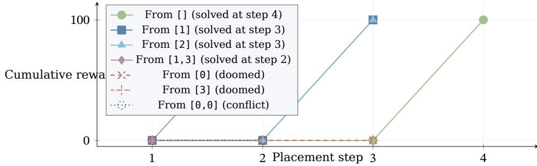
Figure 7: Cumulative reward along the synthesized policy's trajectory for 4-Queens, starting from different partial placements. Valid starts ([], [1], [2], [1,3]) reach the solved state with reward 100; the closer the prefix to a solution, the sooner the reward appears. Doomed starts ([0], [3]) and conflicted starts ([0,0]) flatline at zero—no valid solution is reachable. Every data point is verified by refl .
