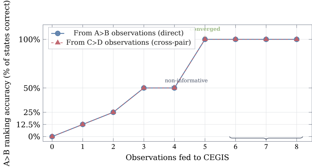
Figure 11: A>B ranking accuracy as C-vs-D (sub-optimal) observations accumulate. The blue circles (direct A>B observations) and red triangles (C>D cross-pair observations) produce identical curves —they overlap exactly. CEGIS receives the same PredObs values regardless of which pair was observed. Step 4 is non-informative (both surviving programs agree at that state). After step 5 the version space has converged; steps 6–8 are redundant. Every data point is verified by refl in Agda.
