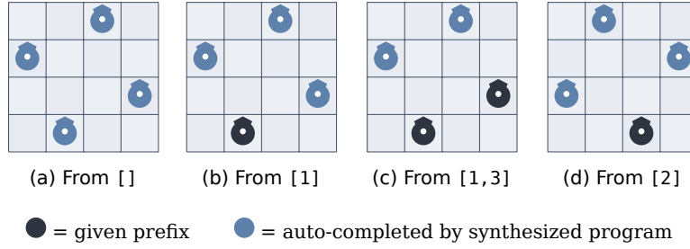
Figure 6: Partial completion by the feature-learned synthesized program. (a) Starting from the empty board, the program discovers solution [1,3,0,2]. (b)-(c) Given a partial optimal placement (dark queens), it correctly completes the remaining positions (blue queens) using only the 6 auto-discovered pair-any features—never seeing these partial boards during training. (d) Starting from a different first queen, it discovers the second valid 4-Queens solution [2,0,3,1]. All results verified by refl.
