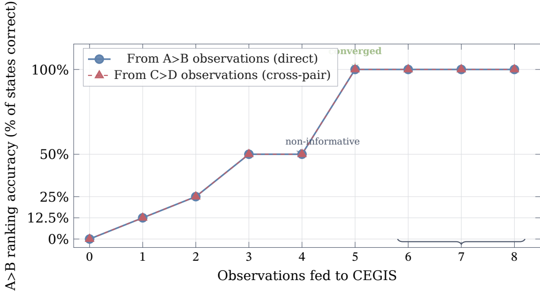
Figure 11: A > B ranking accuracy as C-vs-D (sub-optimal) observations accumulate. The blue circles (direct A > B observations) and red triangles ( C > D cross-pair observations) produce identical curves —they overlap exactly. CEGIS receives the same PredObs values regardless of which pair was observed. Step 4 is non-informative (both surviving programs agree at that state). After step 5 the version space has converged; steps 6–8 are redundant. Every data point is verified by refl in Agda.
