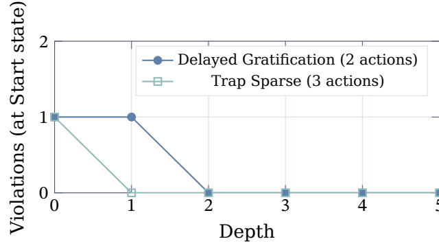
Figure 4: Violations at Start state drop to zero as depth increases. Delayed Gratification requires depth 2 to distinguish equal-immediate-reward paths; Trap Sparse resolves at depth 1. Both are verified in src/CSHRL/Tasks/Classic/ .
