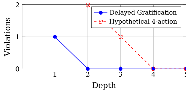
Figure 4: Violations drop to zero as depth increases. Convergence is bounded by |S| \times \binom{|A|}{2} swaps.
