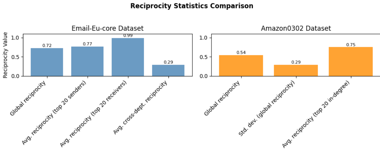
Figure 2: Reciprocity of the network
