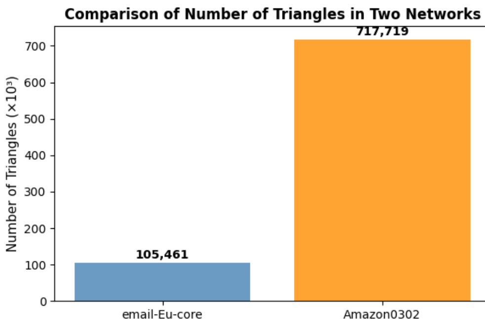
Figure 3: Number of triangles
