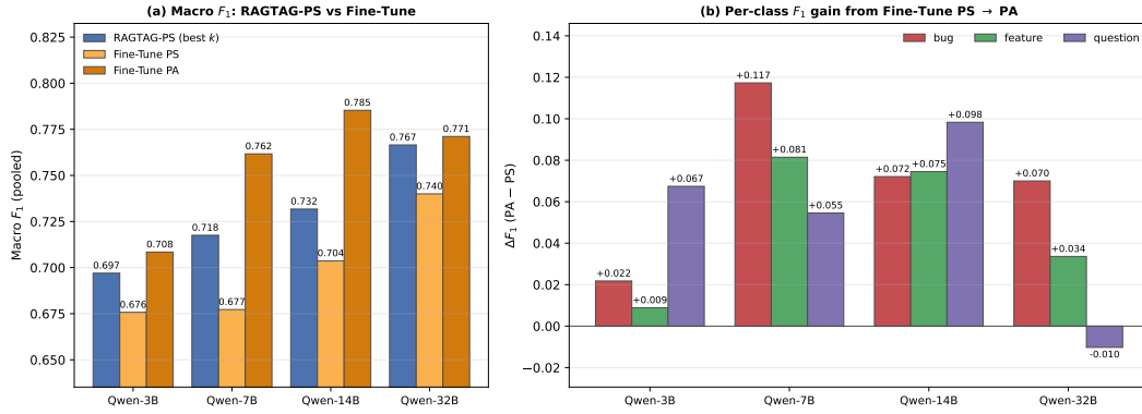
Figure 6 (a) Macro F_1 for RAGTAG at its best k in PS vs Fine-Tune in PS and PA across all four model sizes. (b) Per-class F_1 gain from Fine-Tune PS to Fine-Tune PA ( \Delta F_1 = \text{PA} - \text{PS} ) for each class and model size.
