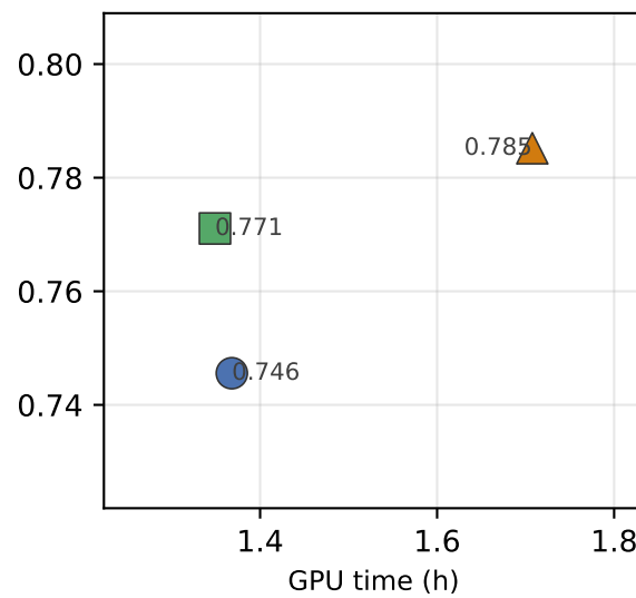
Qwen-14B
