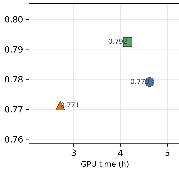
Qwen-32B
