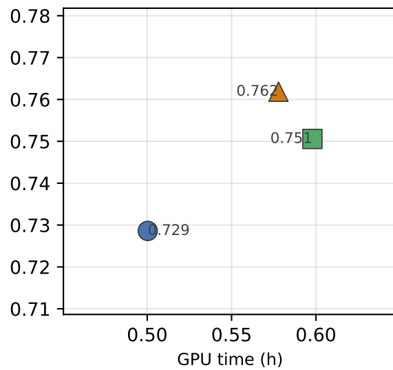
Qwen-7B
