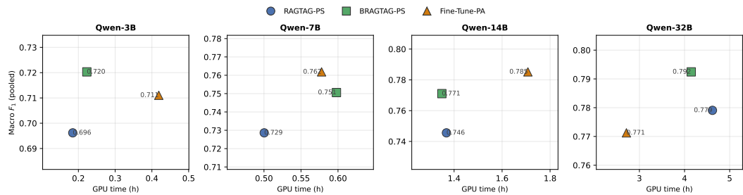
Figure 7 Macro F_1 vs total GPU time at each method’s best configuration, one panel per Qwen size. Each panel uses its own axis range to make the per-model trade-off legible.
