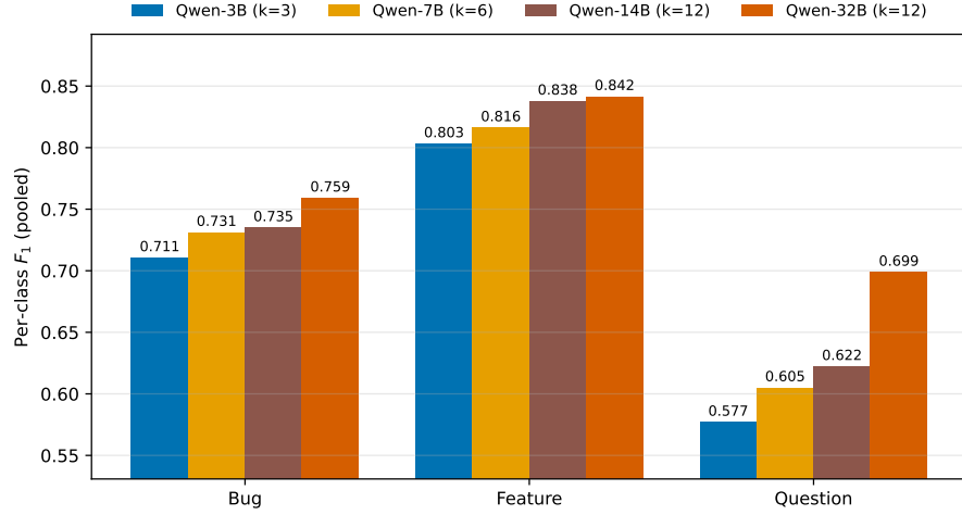
■ Figure 4 Per-class F_1 for each model size at its best RAGTAG-PS configuration.
