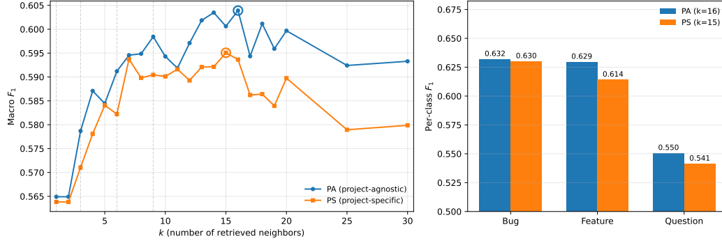
■ Figure 2 (left) VOTAG macro F_1 as a function of k in both PS and PA settings. Circles mark peak performance. (right) Per-class F_1 at each setting's best k ( k=15 for PS, k=16 for PA).
