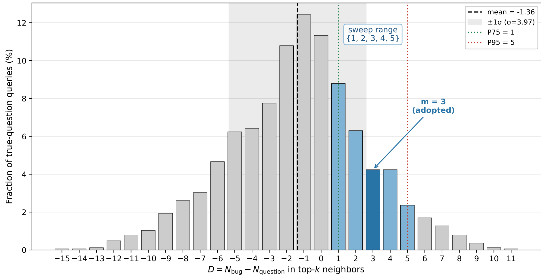
Distribution of D on true-question queries (validation split, pooled k \in [1, 15] )
