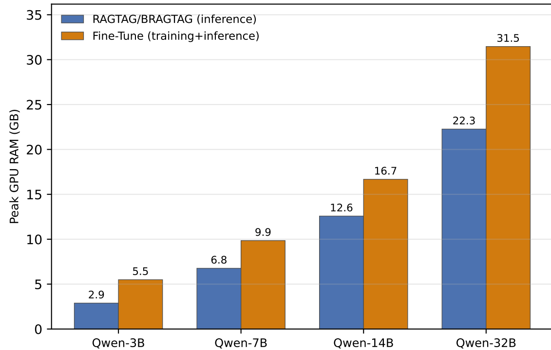
(a) Peak GPU RAM by model size
