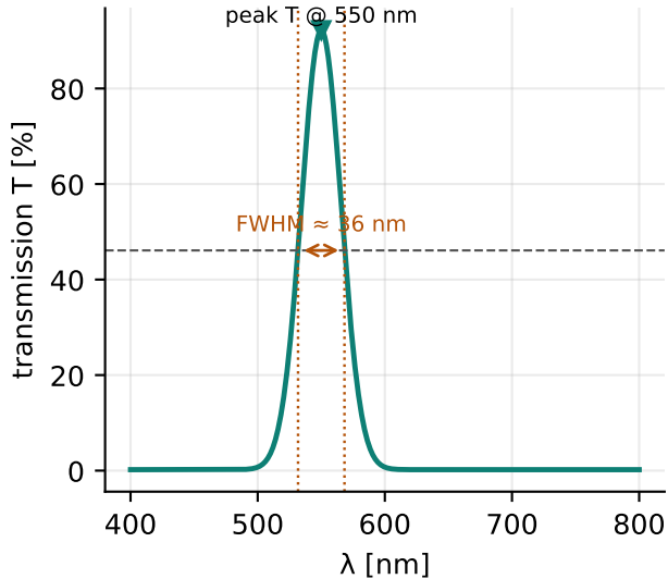
Band-pass filter — transmission
