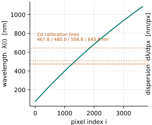
PASCO PS-2600A pixel \rightarrow \lambda (cubic)
