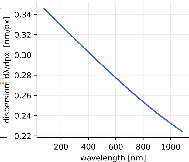
Reciprocal linear dispersion
