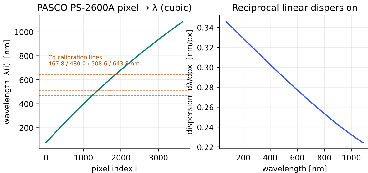
Figure 2: Left: the PASCO pixel→λ cubic with the four Cd calibration lines marked. Right: the reciprocal linear dispersion d\lambda/dpx across the array.
