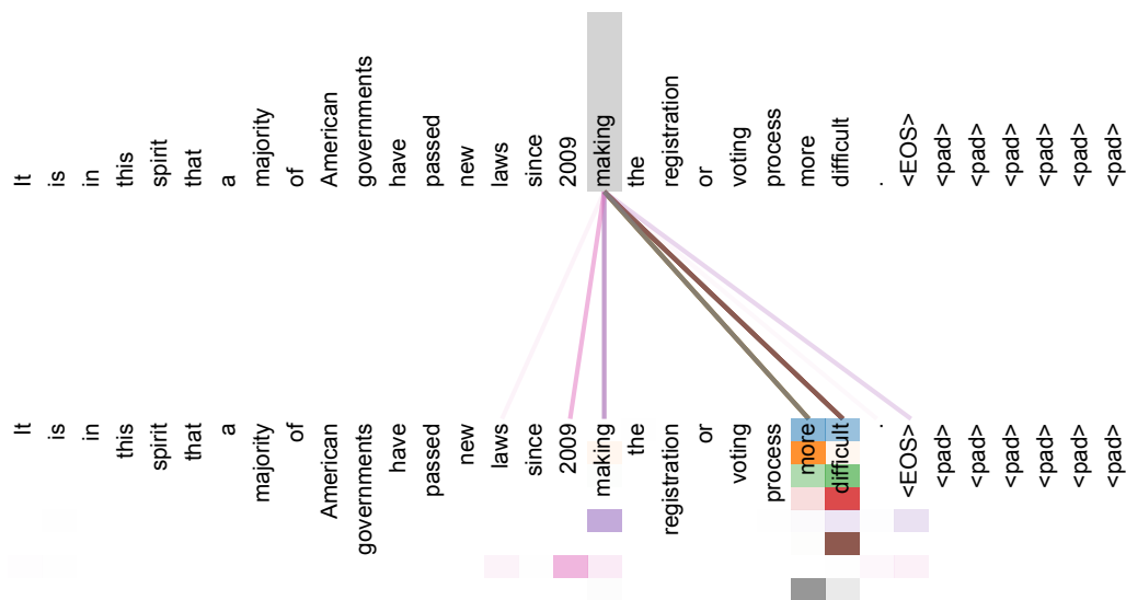
図 9: 長距離依存性に注意力カニズムの例 mechanism following long-distance dependencies in the encoder-decoder for the sentence of 6-7. Many people mentioned heads attend to the distant dependencies in the sentence. The verb and the object are, of course, the main phrase in the sentence. The attention mechanism is shown only for the word and the object. The figure is a head view of the encoder-decoder. The head is viewed in color.
