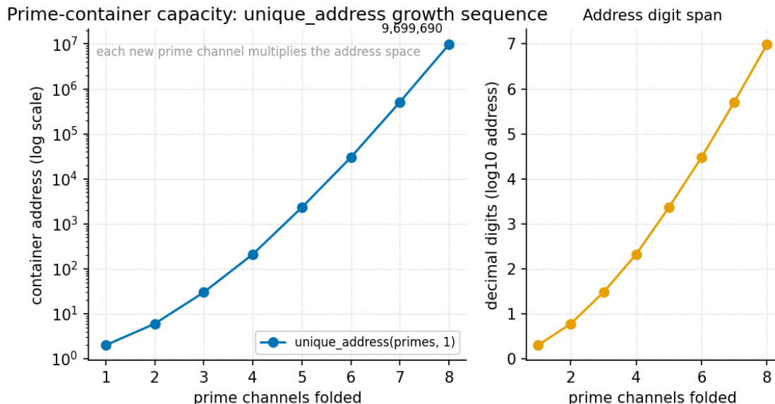
Figure 46. Prime-container capacity: the growth sequence of textbook.models.unique_address as odd-prime vaults join the registry one at a time, each vault contributing an exponent budget of addresses on top of the binary anchor. Every additional vault prime multiplies the number of distinct residue-index addresses rather than adding to it, because each address is the product \prod p_i^{e_i} over the vault primes and their occupancies. The takeaway is the compounding itself — the visual signature of a vault architecture whose encoding is injective and reversible by the fundamental theorem of arithmetic.
