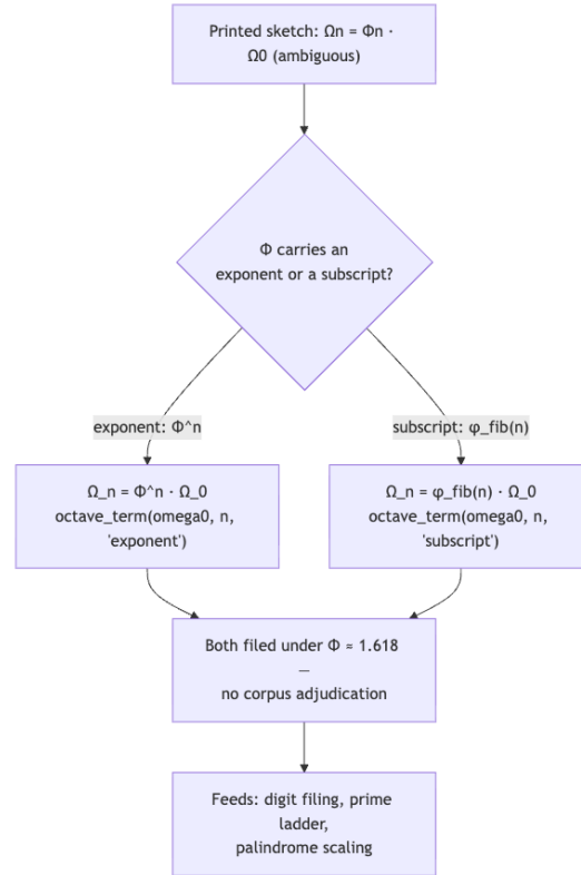
Figure 15. Mermaid diagram
