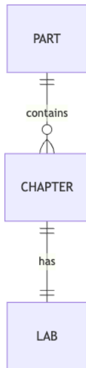
Figure 77. Mermaid diagram
