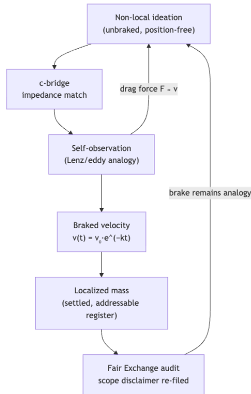
Figure 32. Mermaid diagram
