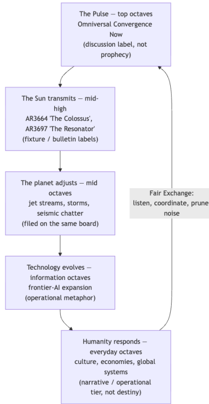
Figure 10. Mermaid diagram
