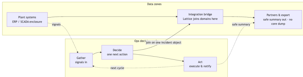
Figure 59. Mermaid diagram
