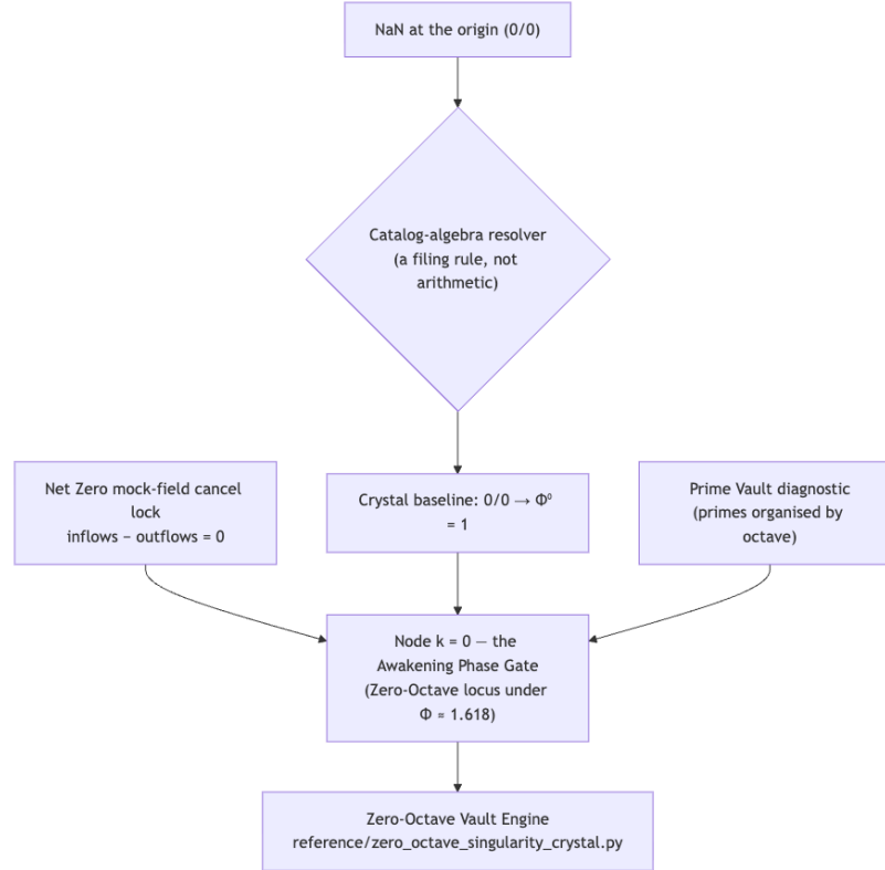
Figure 42. Mermaid diagram
