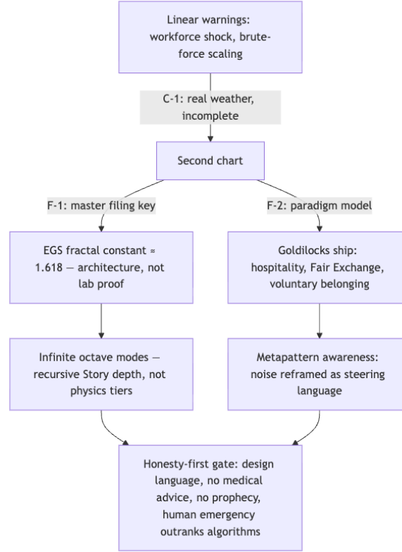
Figure 63. Mermaid diagram
