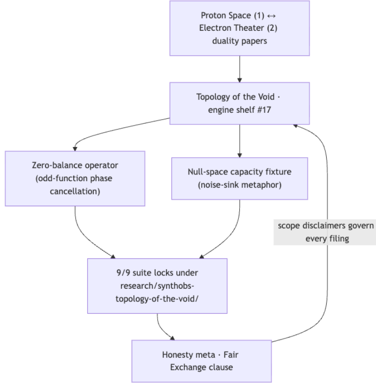
Figure 23. Mermaid diagram
