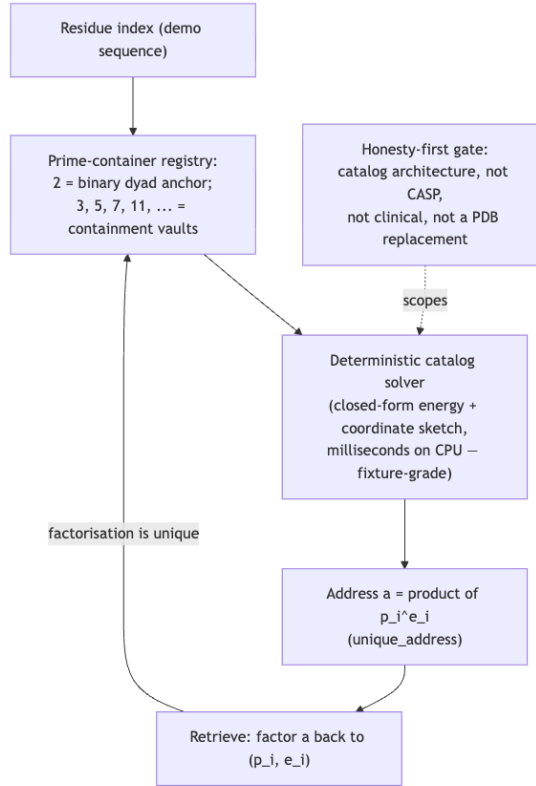
Figure 47. Mermaid diagram
