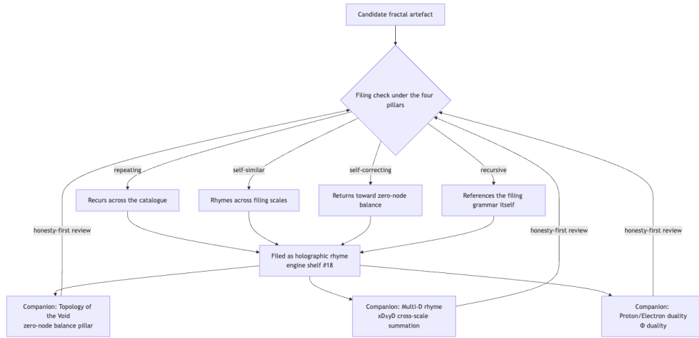
Figure 19. Mermaid diagram
