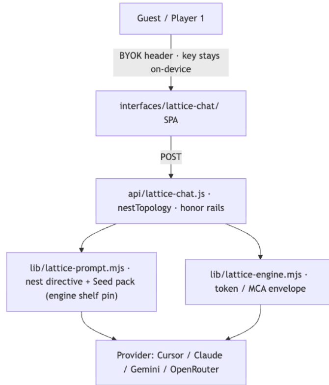
Figure 6. Mermaid diagram
