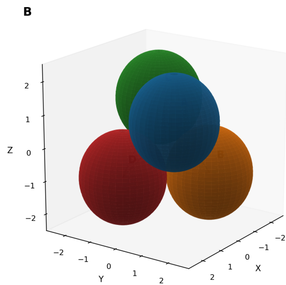
B — Tetrahedron as close-packed spheres (IVM/CCP/FCC)
