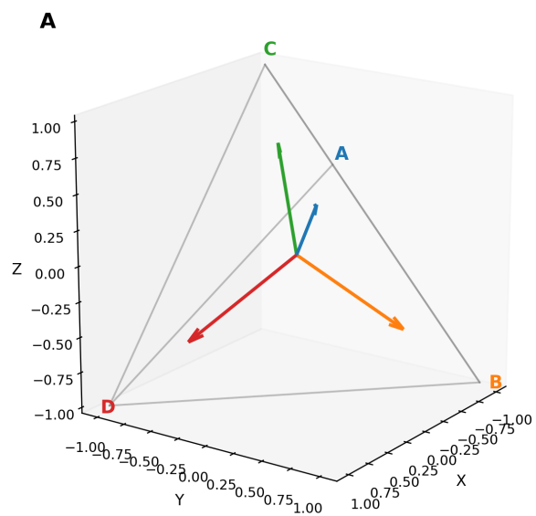
A — Quadray axes (A,B,C,D)
