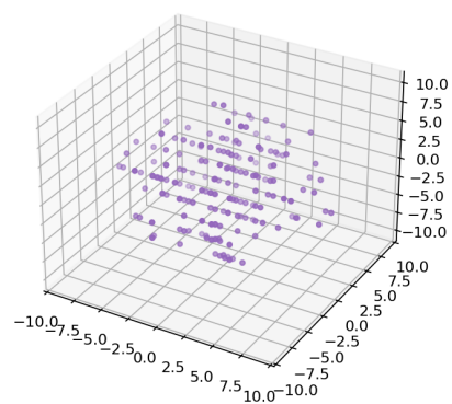
Urner embedding
