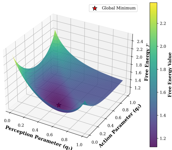
Free Energy Landscape (4D Active Inference Framework)
