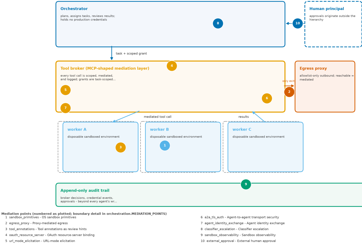
Figure 8: A reference orchestration: one orchestrator delegating through an MCP-style tool broker to three disposable workers, with the ten mediation points numbered at each trust-boundary crossing.
