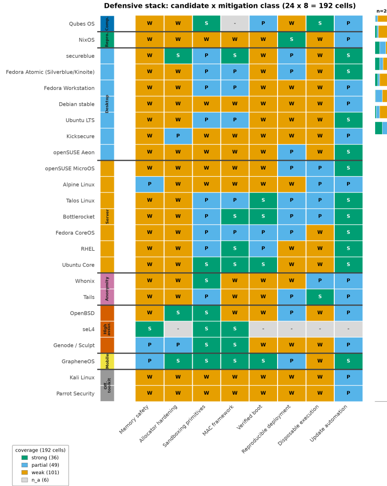
Figure 3: The defensive-stack matrix: 24 candidates scored against eight mitigation classes — memory safety, allocator hardening, sandboxing primitives, MAC framework, verified boot, reproducible deployment, disposable execution, and update automation — using the strong/partial/weak/n_a stance vocabulary, rendered from output/data/defensive_stack.csv with candidate categories grouped and per-class coverage shown as a marginal bar.
