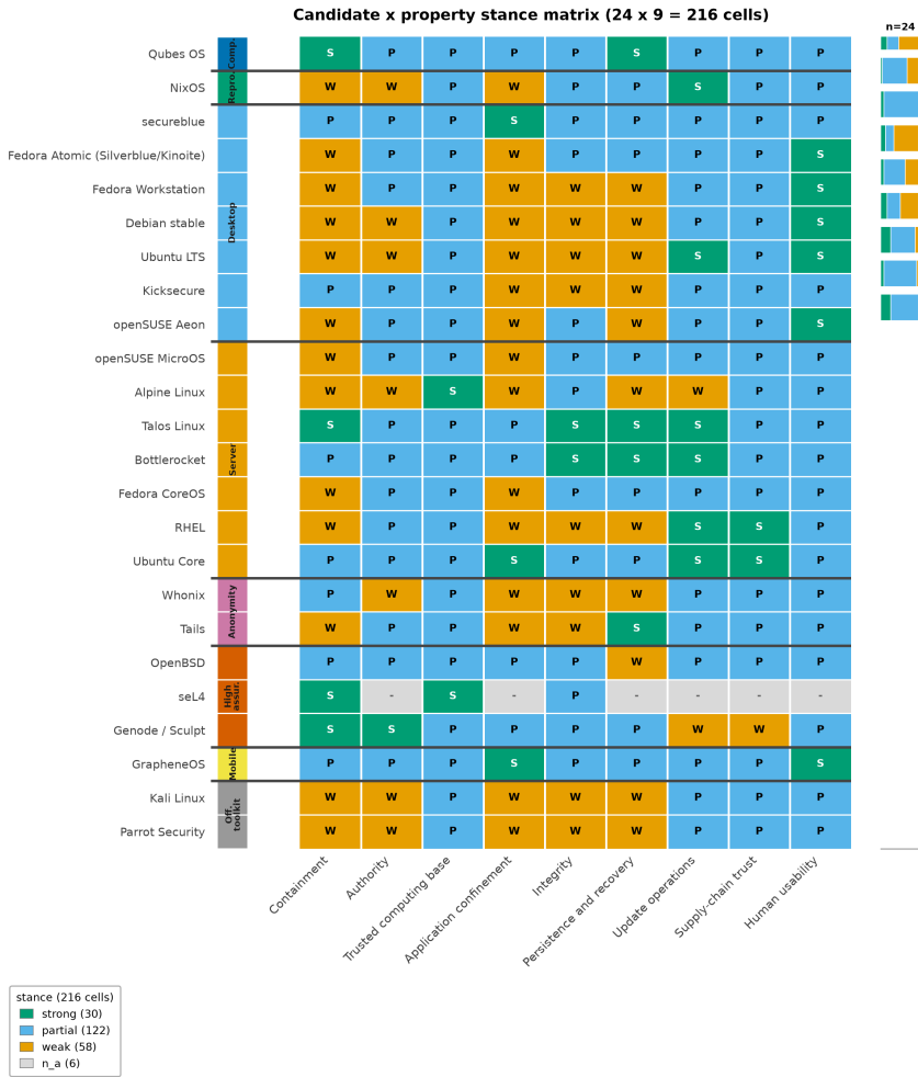
Figure 2: The candidate–property stance matrix across 24 candidates and 9 properties, rendered from output/data/evaluation_matrix.csv with colorblind-safe encoding of the strong/partial/weak/n_a vocabulary.
