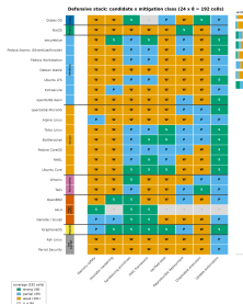
Figure 2: The defensive-stack matrix: 24 candidates scored against eight mitigation classes — memory safety, allocator hardening, sandboxing primitives, MAC framework, verified boot, reproducible deployment, disposable execution, and update automation — using the strong/partial/weak/n_a stance vocabulary, rendered from output/data/defensive_stack.csv with candidate categories grouped and per-class coverage shown as a marginal bar.
