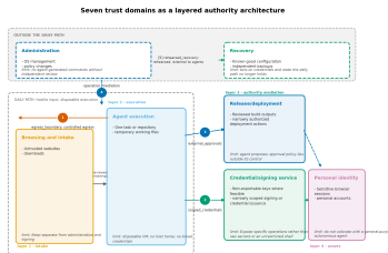
Figure 1: The seven trust domains of the proposed agentic authority architecture and the boundaries between them. Administration, personal identity, and the credential service hold assets whose loss is not recoverable by rebuilding; agent execution and browsing/intake meet hostile input and are deliberately disposable; release/deployment mediates what leaves; recovery sits beyond the destructive authority of everything else. The architecture's objective is real separation of authority, not maximizing the number of compartments.
