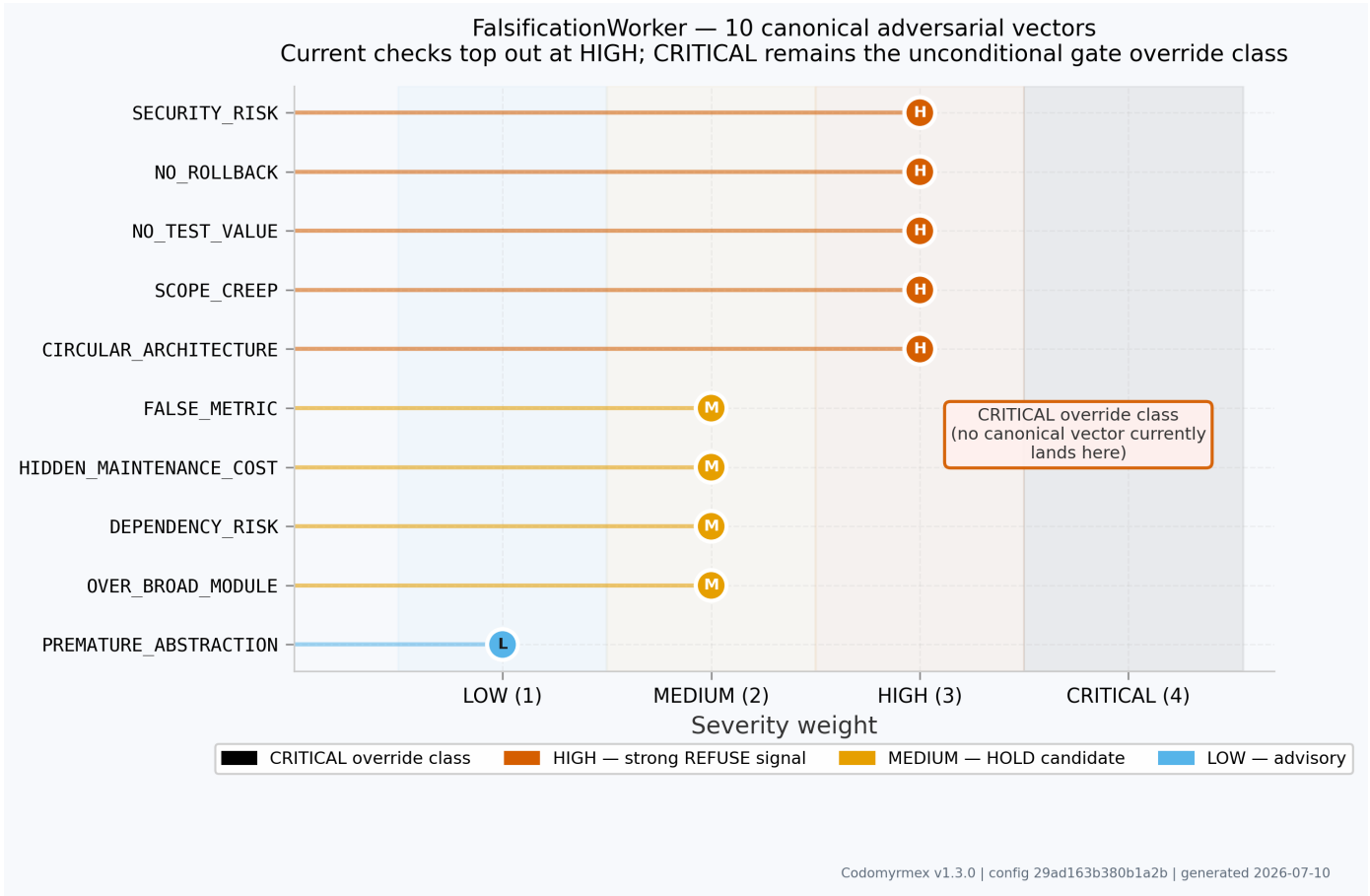
Figure 3: Falsification worker: 10 canonical adversarial attack vectors ordered by severity weight (HIGH=3, MEDIUM=2, LOW=1). Colour encodes severity class. The adversarial worker applies all 10 checks to every ActionProposal ; the empty CRITICAL band is shown as the gate override class for findings that must issue unconditional REFUSE before scoring.
