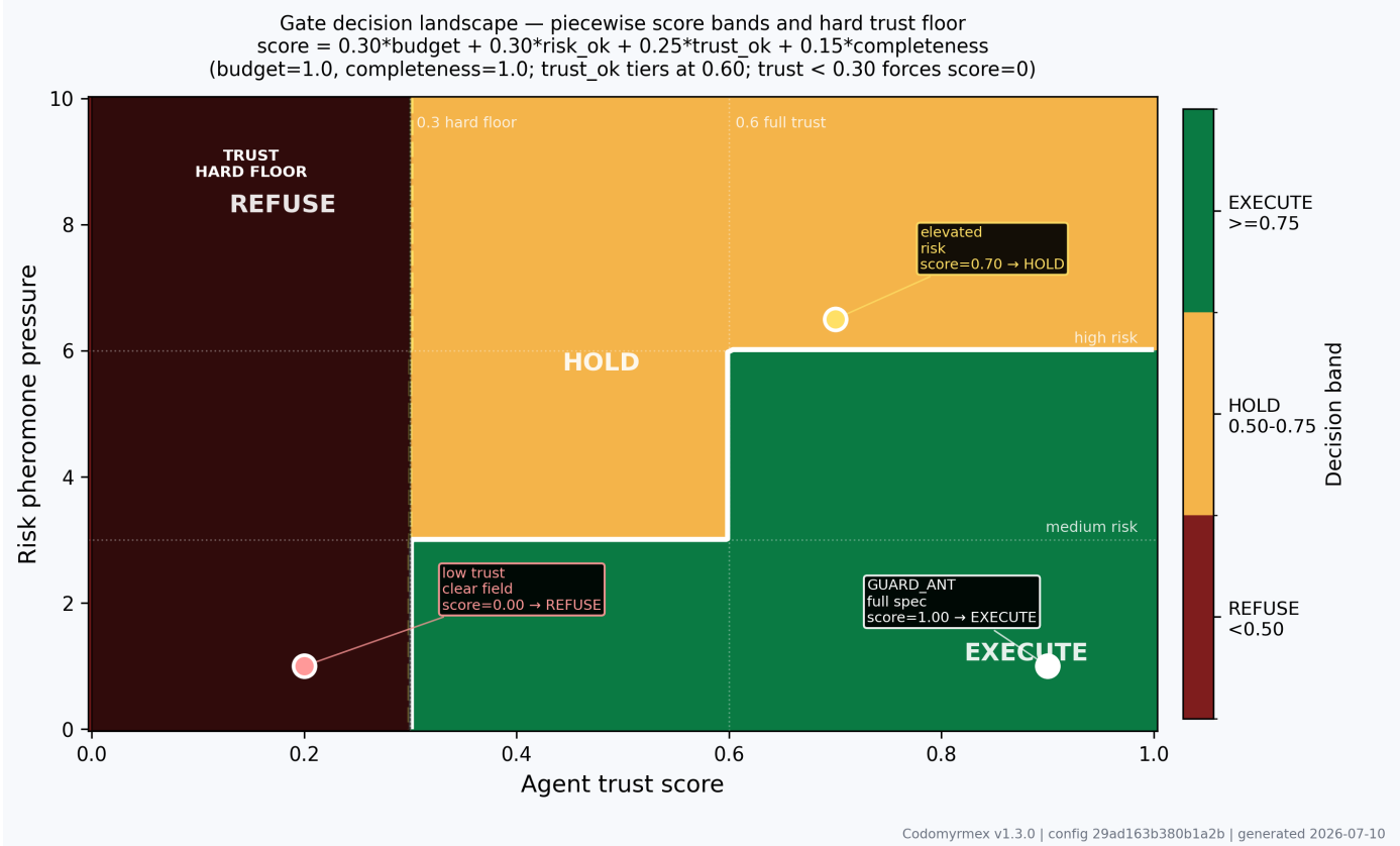
Figure 6: Gate decision landscape across the (trust score, risk pheromone pressure) parameter space. Green regions indicate EXECUTE (score \geq 0.75 ); yellow/amber regions indicate HOLD ( 0.50 \leq \text{score} < 0.75 ); red regions indicate REFUSE (score < 0.50 ). Contour lines mark the two decision boundaries. Budget=1.0 and completeness=1.0 are held constant to isolate the tiered trust and risk-pressure interaction. The solid black strip at trust < 0.30 represents the gate hard-refuse floor: score is forced to 0.0 regardless of all other factors.
