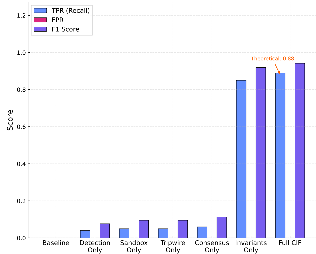
A. Single-Mechanism vs. Full-Pipeline Detection (abla Param) B. Parametric Simulation: Detection Rate by Attack Type (95% Wilson CI; not a deployed model)
