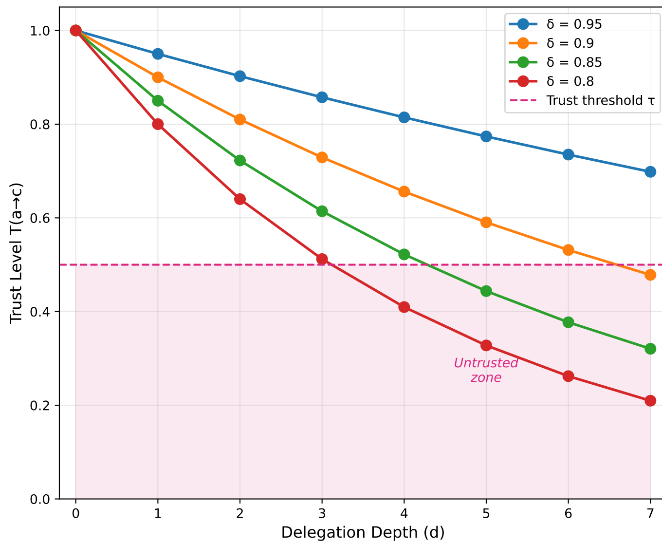
C. Bounded Delegation Chain (Theorem 3.1)
