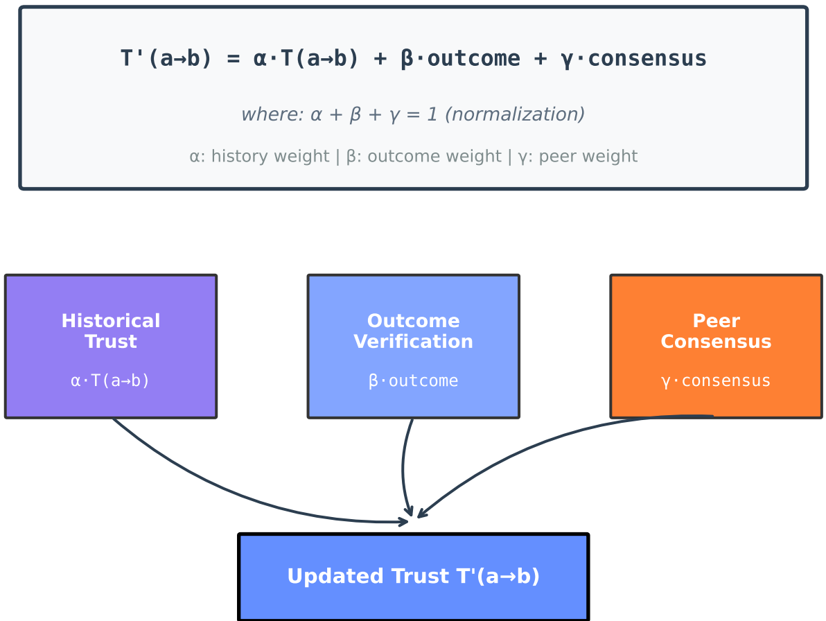
B. Trust Update Mechanism
