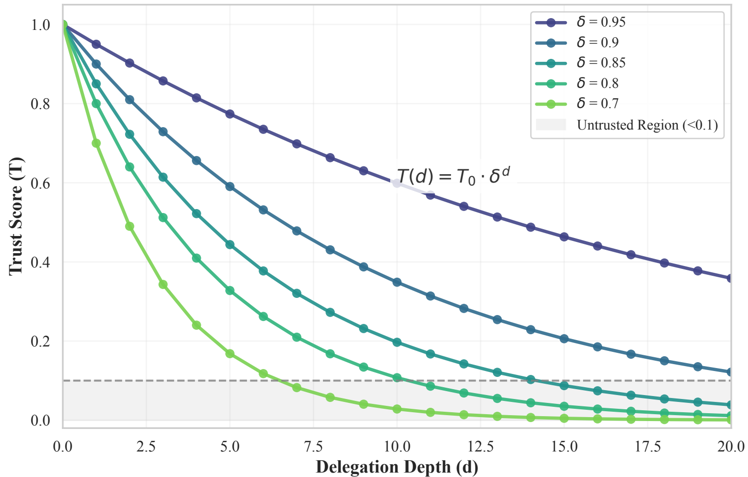
A. Trust Decay Over Delegation Depth
