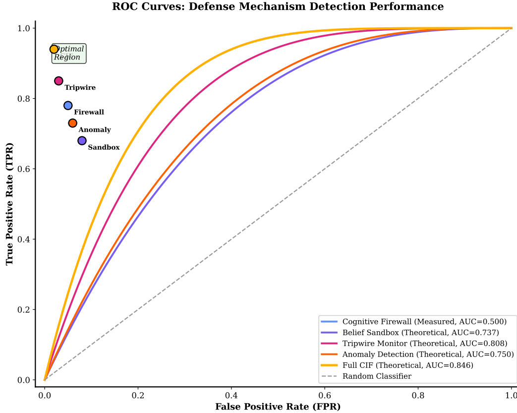
Figure 15: Receiver Operating Characteristic (ROC) curves for CIF detection across attack categories (illustrative/schematic operating points under the Neyman-Pearson framework; the sandbox/tripwire/anomaly/full-CIF curves are labeled Theoretical, not empirical measurements, whereas the Cognitive Firewall entry is measured over this part’s small test corpus. That entry is a single operating point at zero false positives, drawn as the conventional vertical segment, so the area beside it equals its true-positive rate and must not be read as chance performance despite coinciding numerically with the random-classifier diagonal. Measured evaluation curves are reported in Part 2).
