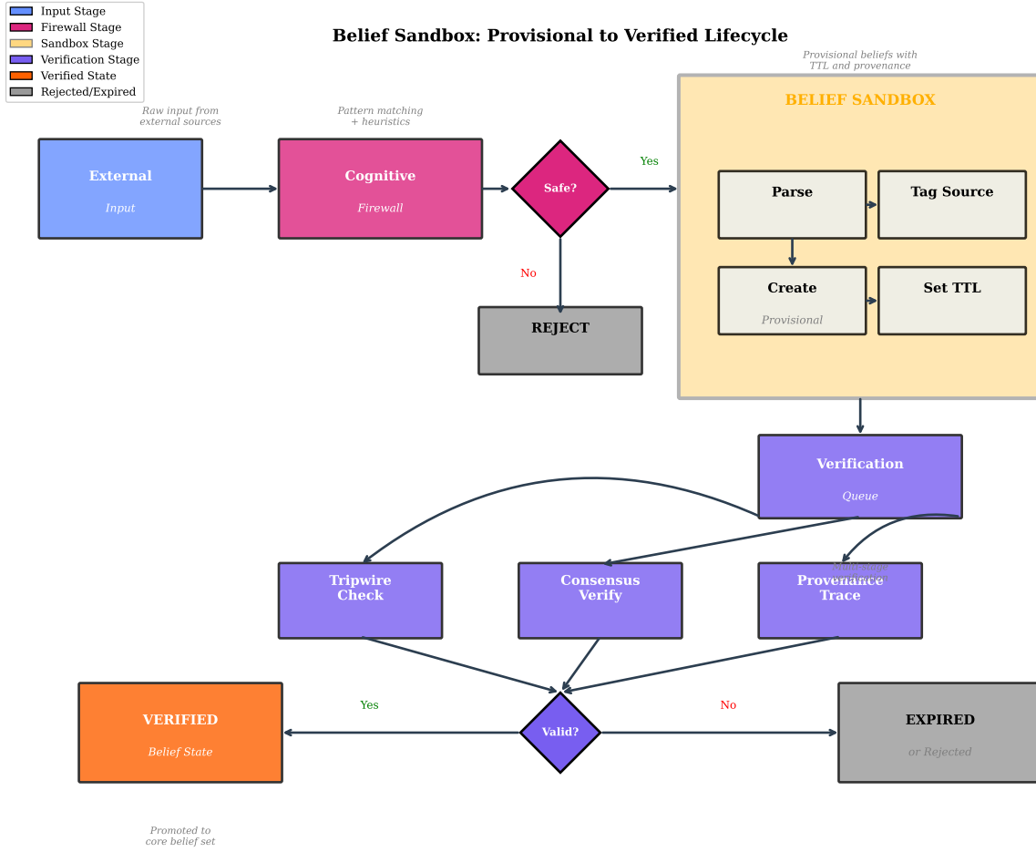
Figure 12: Belief Sandbox Architecture
