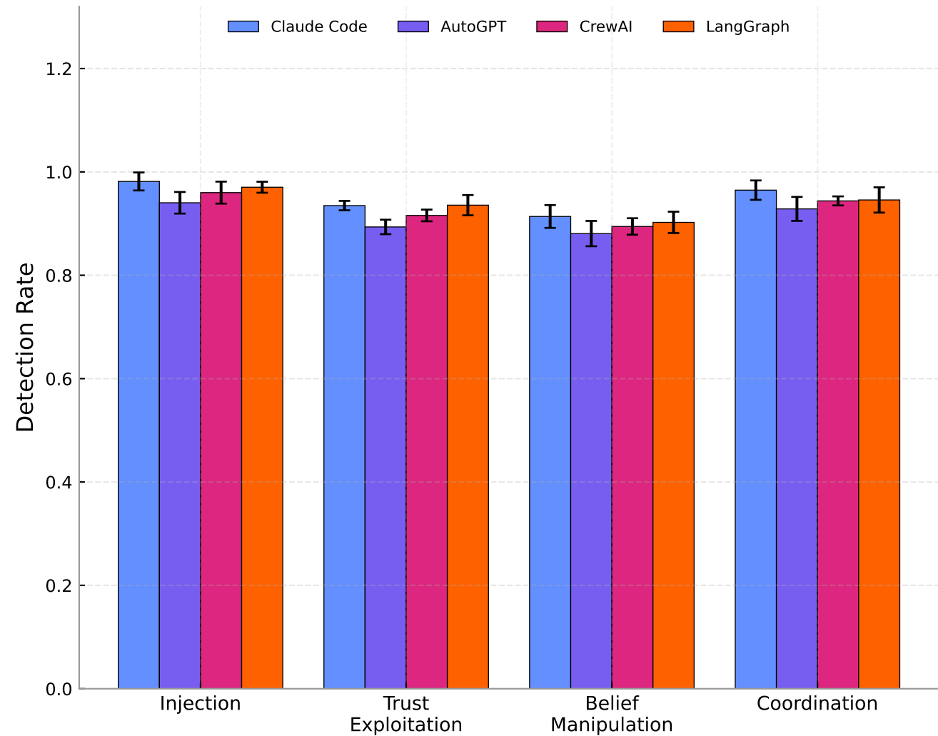
B. Measured Detection Rate by Attack Type and Architecture
