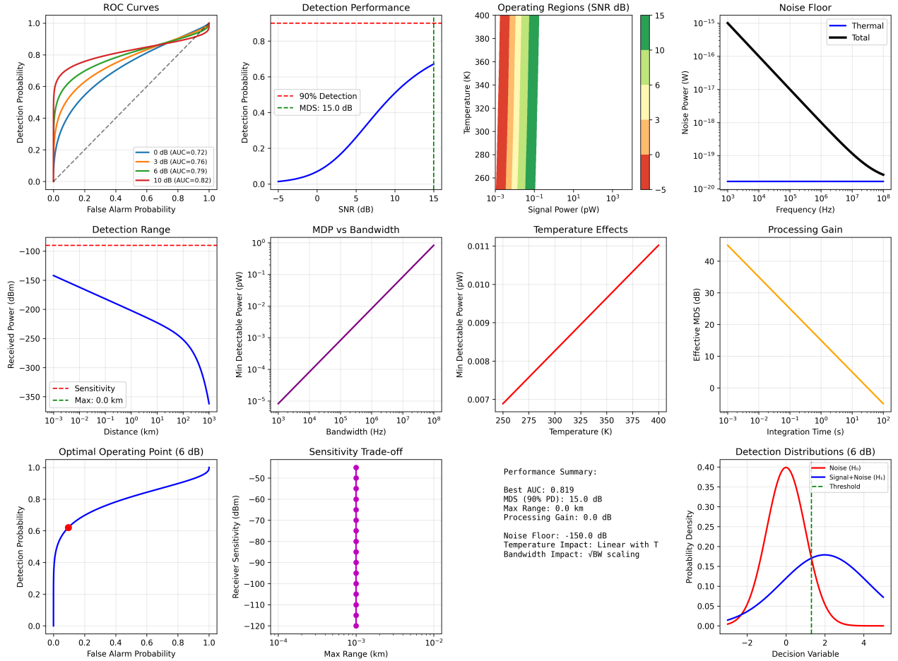
Figure 2: Detection limits and operating regions generated by 'scripts/generate_detection_limits.py' using 'src/case_studies/detection_limits.py' . Panel shows ROC curves, detection performance
