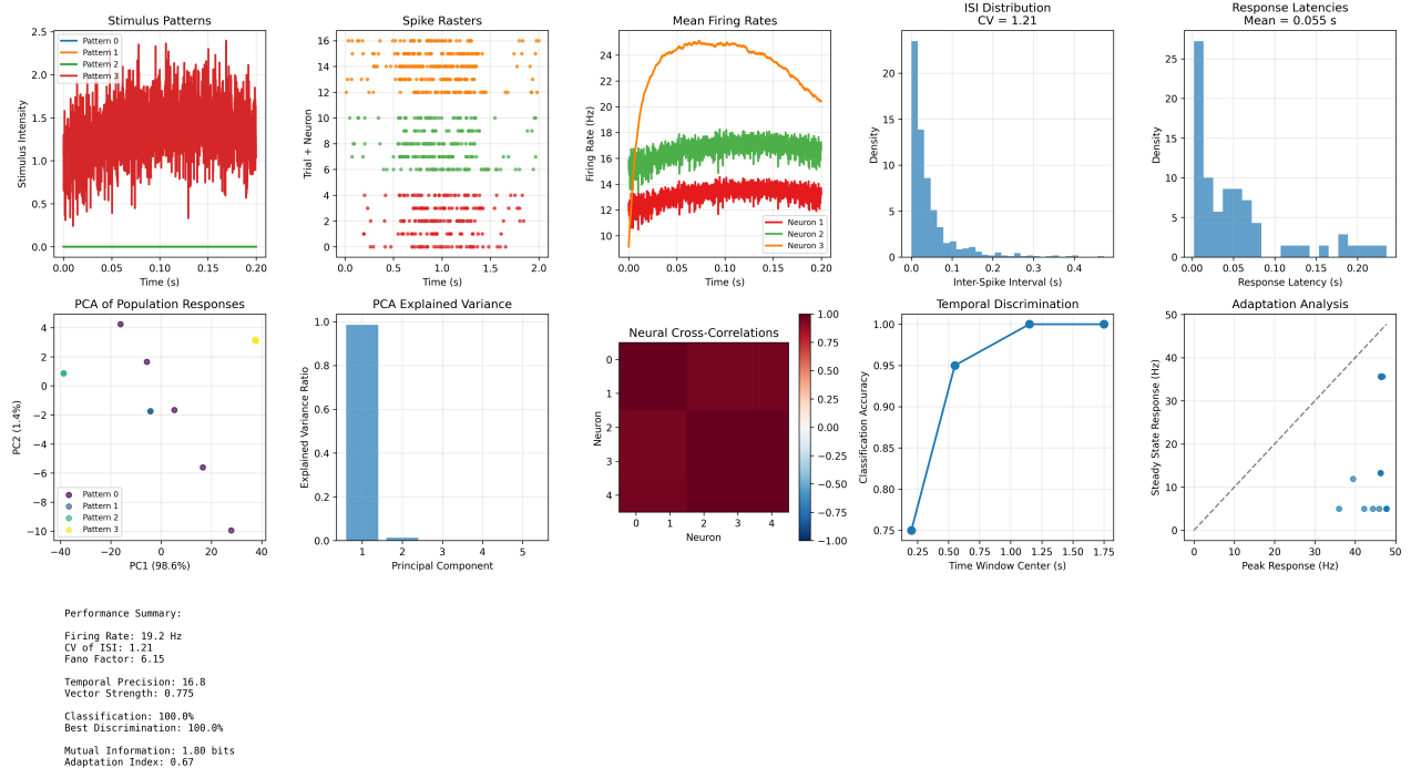
Figure 1: Neural encoding analyses generated deterministically by ‘scripts/generate_neural_encoding_analysis.py’ using ‘src/case_studies/neural_encoding.py’. Panels include spike trains, temporal
