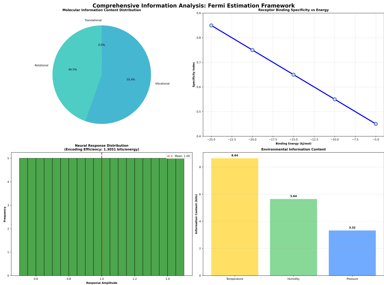
Figure 2: Integrated information analysis (from 'scripts/generate_integrated_analysis.py') showing molecular, receptor, neural and environmental information decomposition in domain information balances.
