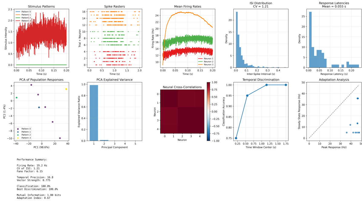
Figure 8: Neural encoding analyses generated deterministically by ‘scripts/generate_neural_encoding_analysis.py’ using ‘src/case_studies/neural_encoding.py’. Panels include spike trains, temporal discrimination, and adaptation analysis.
