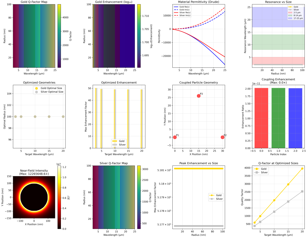
Figure 13: Plasmonic geometry sweep produced deterministically by ‘scripts/generate_plasmonic_geometry_sweep.py’ using ‘src/case_studies/plasmonic_geometry.py’. Panels show Drude perm
