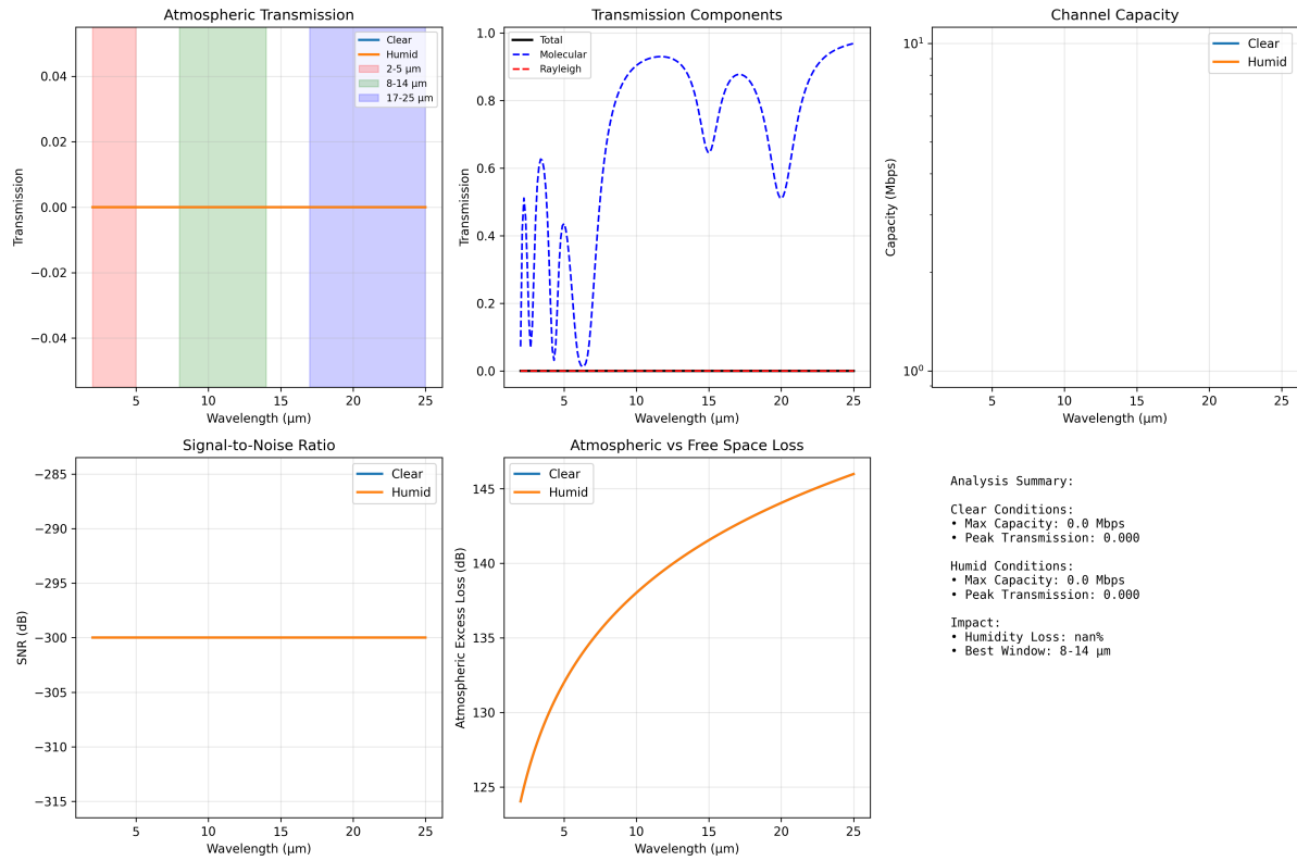
Figure 3: Comprehensive environmental channel outputs produced deterministically by 'scripts/generate_environmental_channel_analysis.py' using 'src/case_studies/environmental_channel.py'. Panelsshowmo
