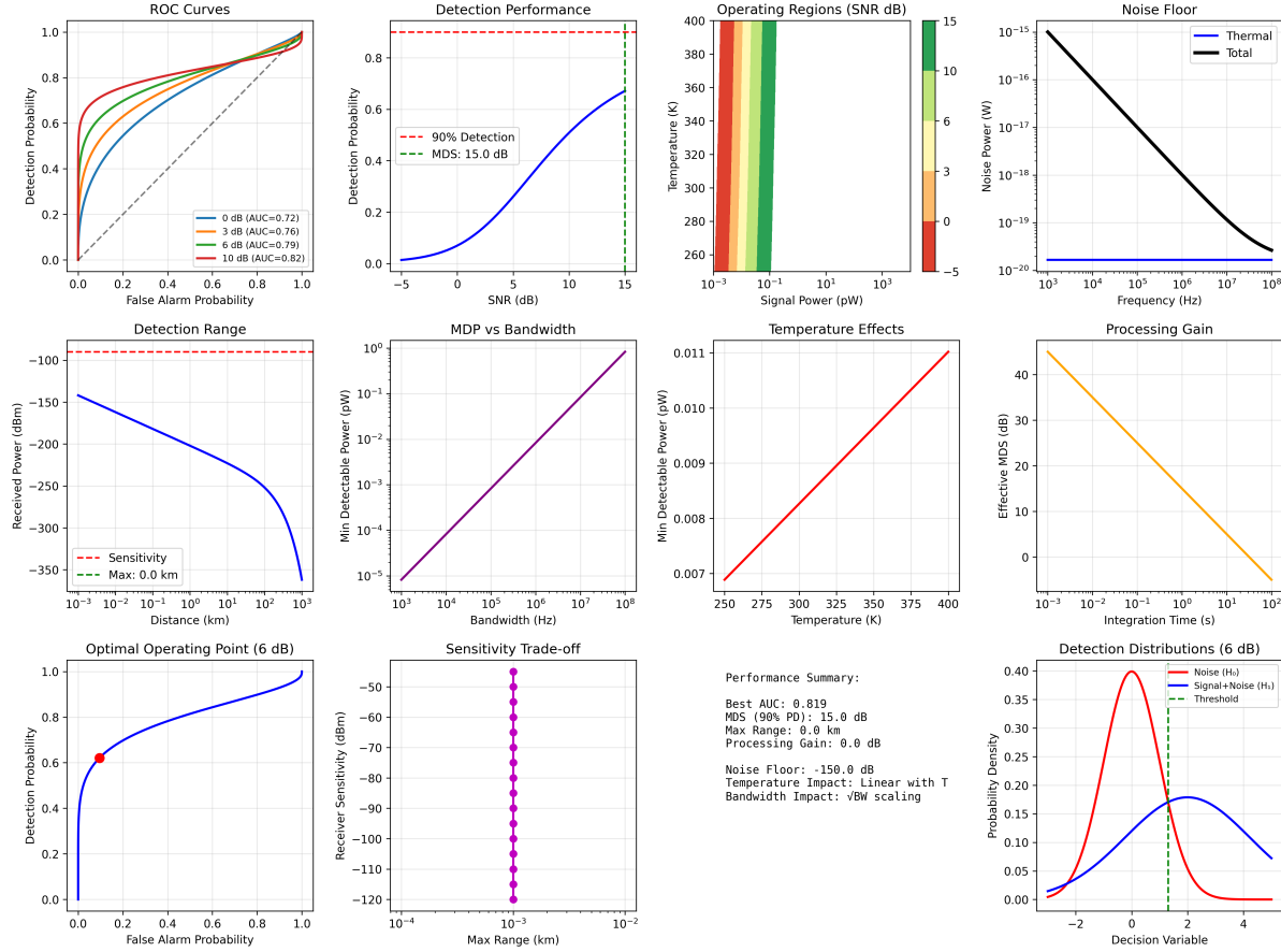
Figure 6: Comprehensive detection analysis: ROC curves with AUC metrics, detection performance vs SNR showing minimum detectable signal (MDS), operating regions in power-temperature space, noise-floor components, detection range analysis, and parameter optimization. Includes processing gain effects, optimal threshold selection, and performance trade-offs for IR olfactory detection systems.
