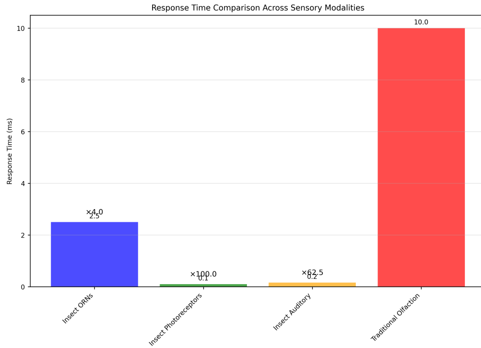
Figure 71: Response time comparison across sensory modalities.
