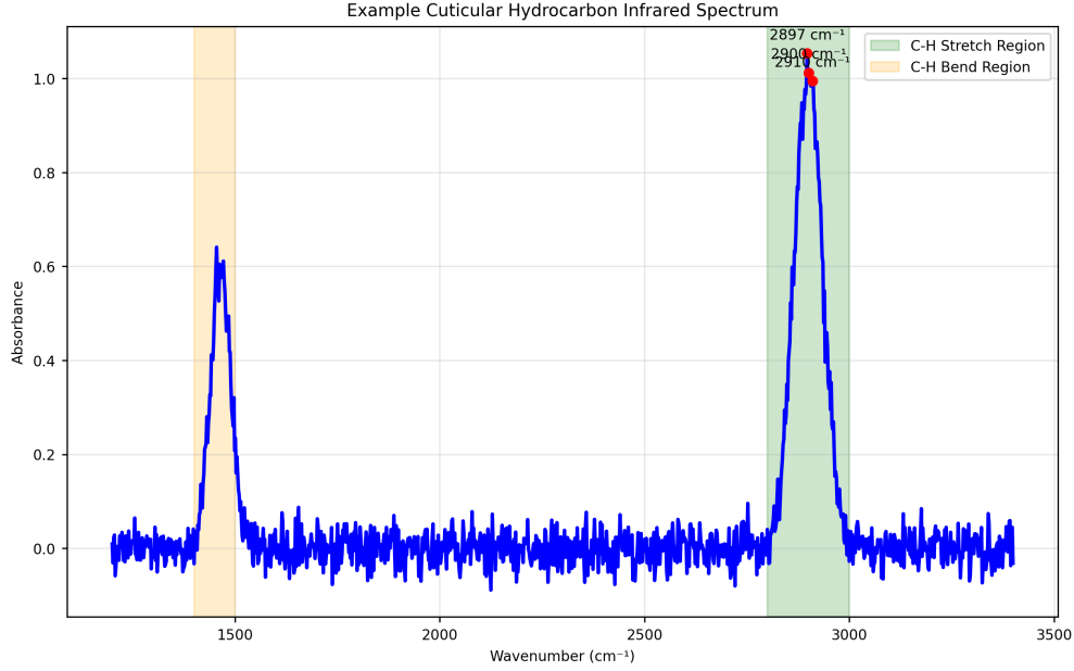
Figure 22: Example cuticular hydrocarbon (CHC) spectra showing characteristic infrared emission peaks. Different insect species exhibit distinct spectral signatures that can be used for identification and behavioral analysis. Generated using tested spectroscopic analysis algorithms with peak detection sensitivity of \pm 0.1 m.
