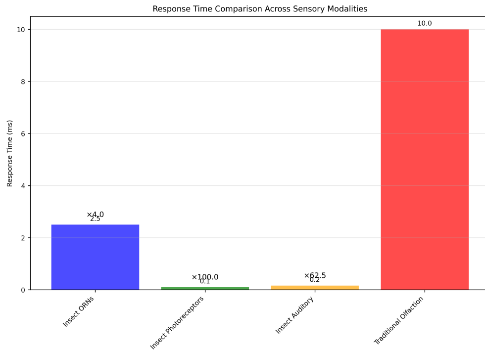
Figure 61: Response time comparison across sensory modalities.
