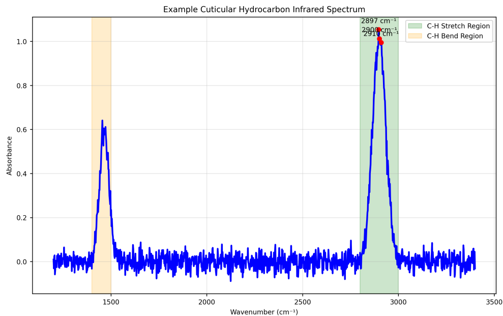
Figure 20: Deterministic synthetic CHC spectrum with C–H stretch and bend regions for illustration.
