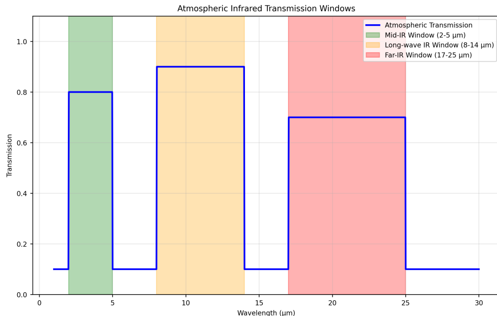
Figure 5: Atmospheric IR transmission windows computed via src.core.calculate_atmospheric_transmission across 1~30μm.
