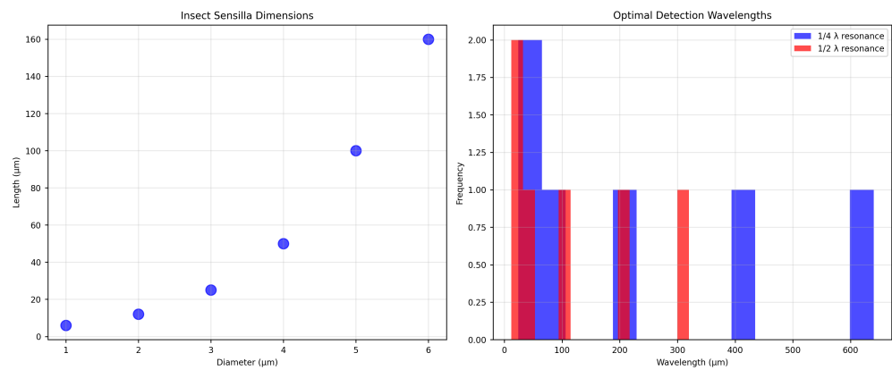
Figure 66: Sensilla dimensions and implied quarter/half-wavelength resonances via src.sensilla.analyze_sensilla_dimensions .
