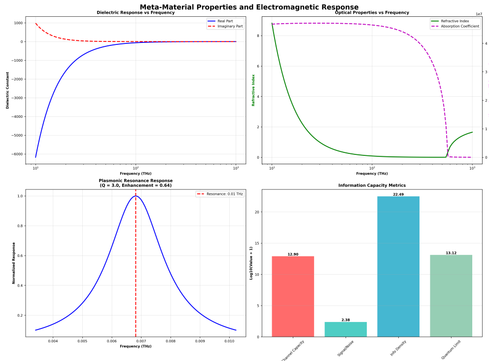
Figure 3: Dielectric response, refractive index/absorption, plasmonic resonance, and info capacity.
