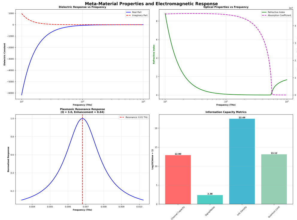
Figure 25: Dielectric response, refractive index/absorption, plasmonic resonance, and info capacity.
