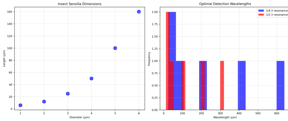
Figure 46: Sensilla dimensions and implied quarter/half-wavelength resonances via src.sensilla.analyze_sensilla_dimensions .
