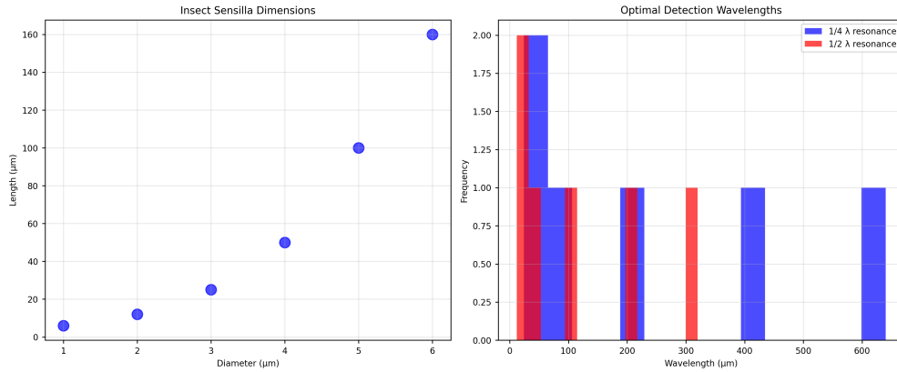
Figure 24: Sensilla dimensions and implied quarter/half-wavelength resonances via src.sensilla.analyze_sensilla_dimensions .
