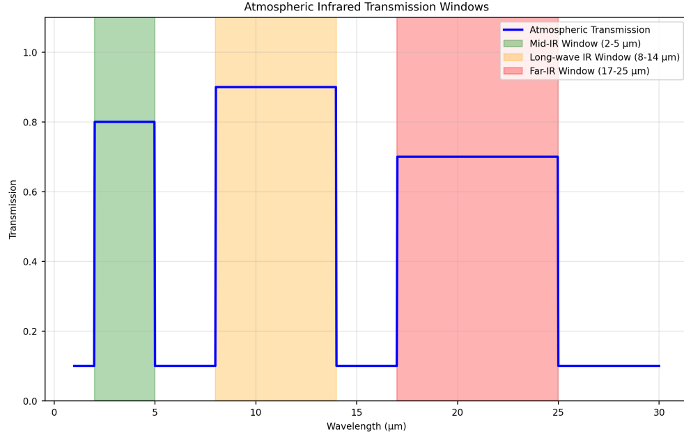
Figure 15: Atmospheric IR transmission windows computed via src.core.calculate_atmospheric_transmission across 1~30m.
