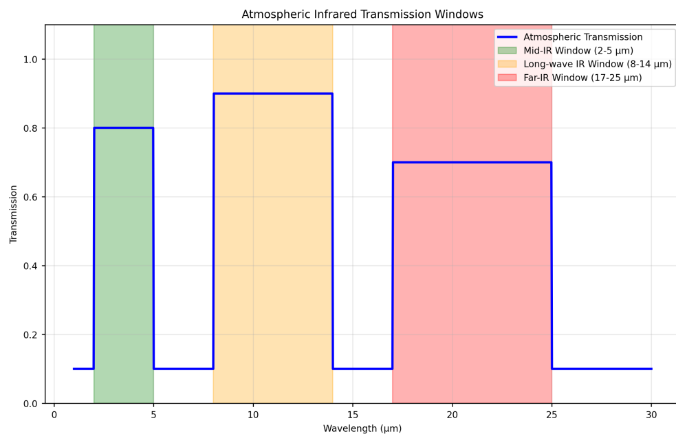
Figure 49: Atmospheric IR transmission windows computed via src.core.calculate_atmospheric_transmission across 1~30m.
