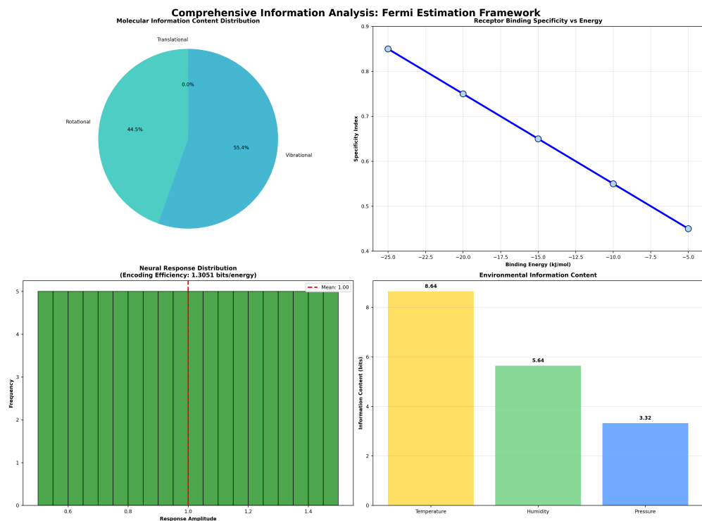
Figure 4: Information content distribution, receptor specificity, neural encoding, and environmental bits.
