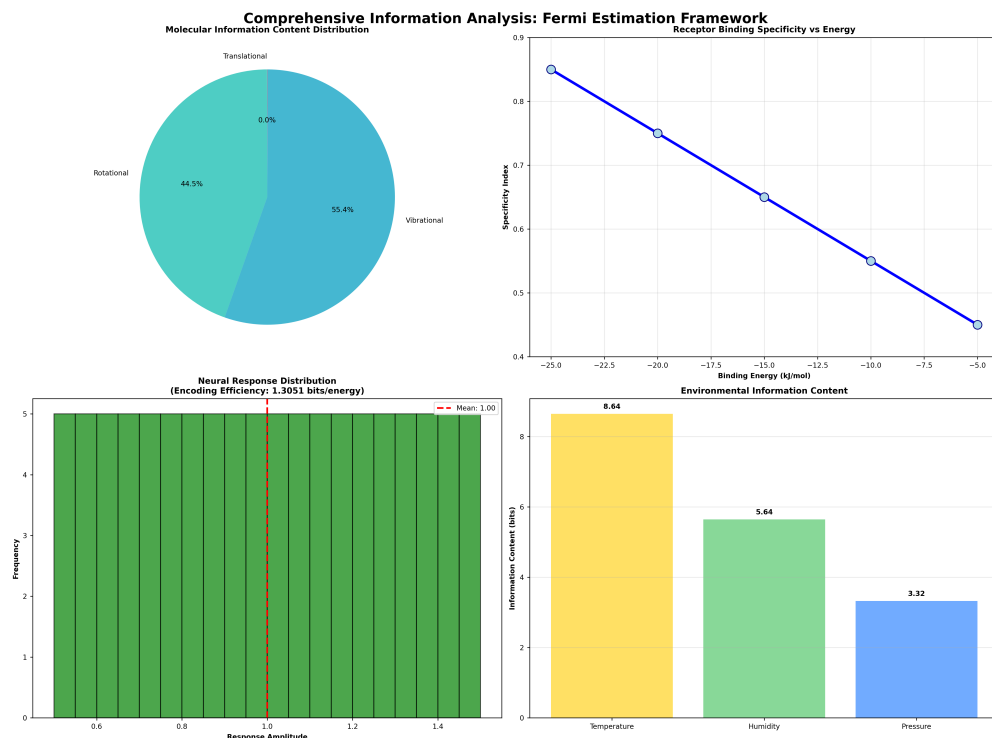
Figure 26: Information content distribution, receptor specificity, neural encoding, and environmental bits.
