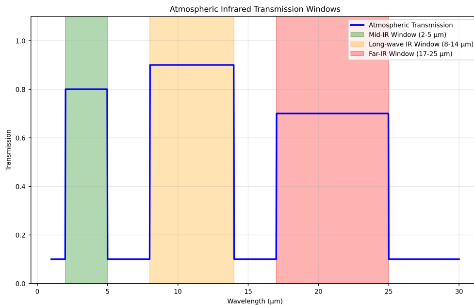
Figure 21: Atmospheric transmission windows in the infrared range, showing optimal wavelengths for insect semiochemical detection. The Earth’s atmosphere has specific transmission windows (2-5 m, 8-14 m, 17-25 m) that correspond closely to the emission spectra of insect semiochemicals. Generated using tested computational models implementing empirical atmospheric data.
