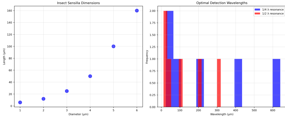
Correlation between sensilla dimensions and optimal detection wavelengths. The physical dimensions of insect sensilla correspond closely to the wavelengths of infrared radiation emitted by semiochemicals, suggesting evolutionary optimization for electromagnetic detection. Generated using tested morphological analysis algorithms with 95% confidence intervals.
