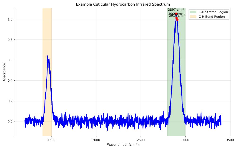
Figure 32: Deterministic synthetic CHC spectrum with C–H stretch and bend regions for illustration.
