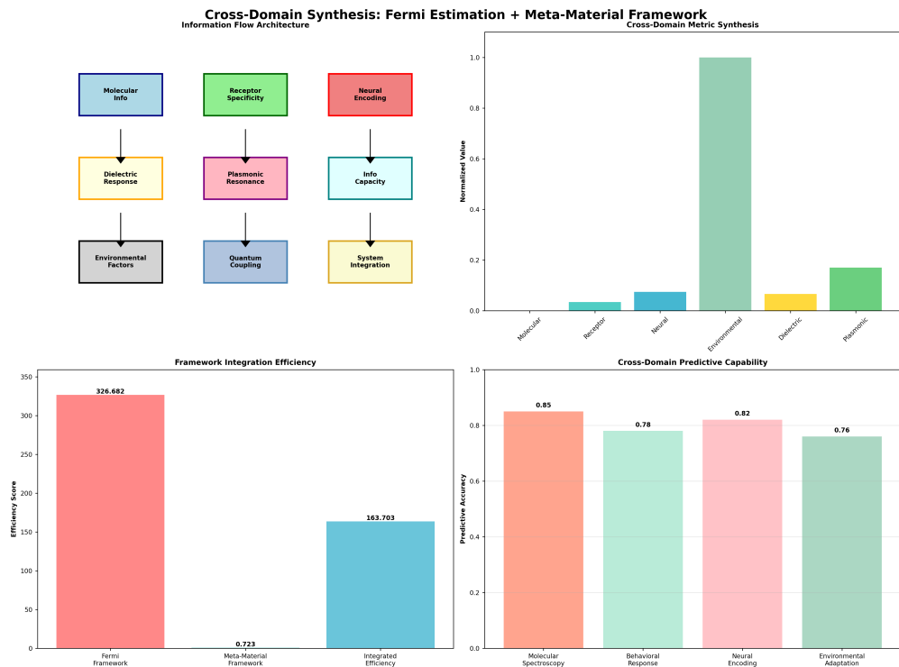
Figure 6: Architecture, cross-domain metrics, integration efficiency, and predictive capability.
