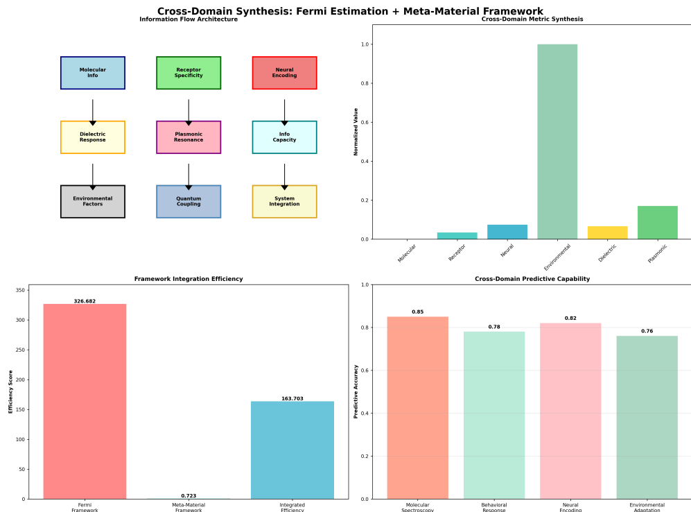
Figure 16: Architecture, cross-domain metrics, integration efficiency, and predictive capability.
