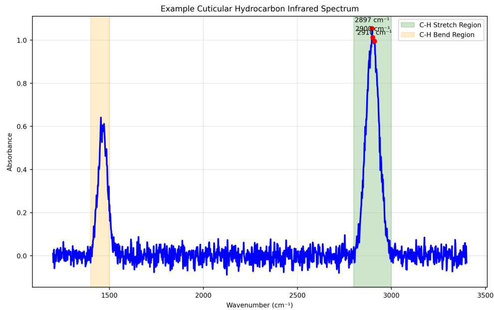
Figure 84: Deterministic synthetic CHC spectrum with C–H stretch and bend regions for illustration.
