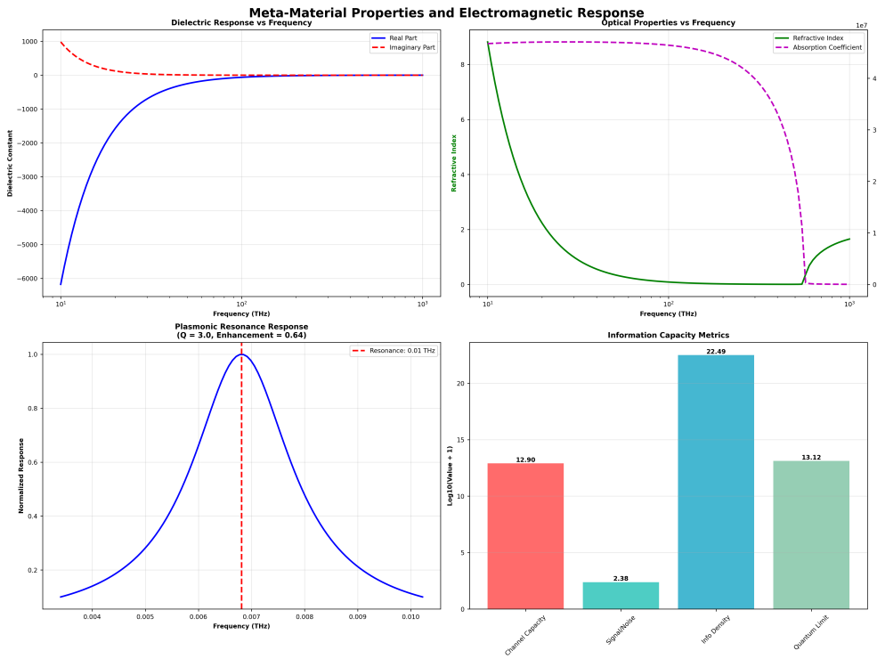
Figure 37: Dielectric response, refractive index/absorption, plasmonic resonance, and info capacity.
