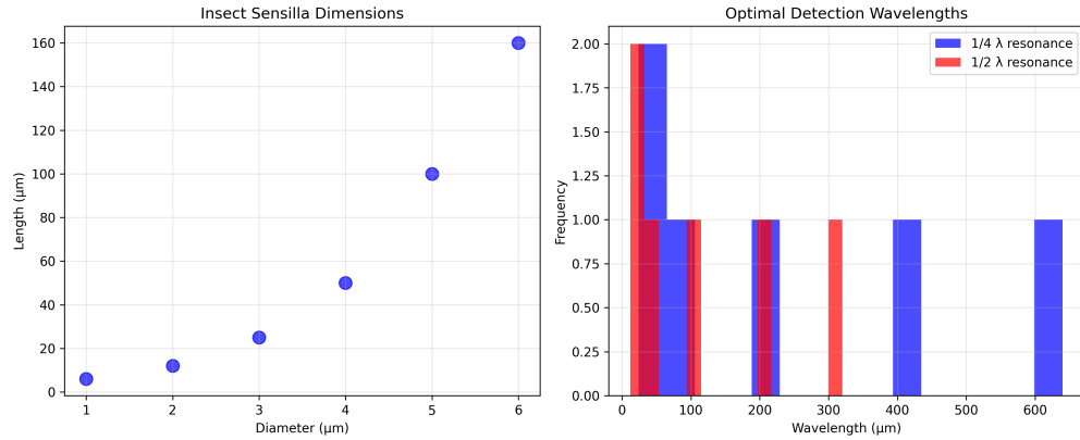
\caption{Correlation between sensilla dimensions and optimal detection wavelengths. The physical dimensions of insect sensilla correspond closely to the wavelengths of infrared radiation emitted by semiochemicals, suggesting evolutionary optimization for electromagnetic detection. Generated using tested morphological analysis algorithms with 95% confidence intervals.} \end{figure}
